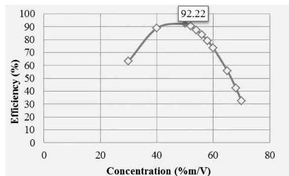
Figure 4. Graphical representation of polynomial regression for concentrations greater than 50% m/V at 100 ppm dose in synthetic brine
