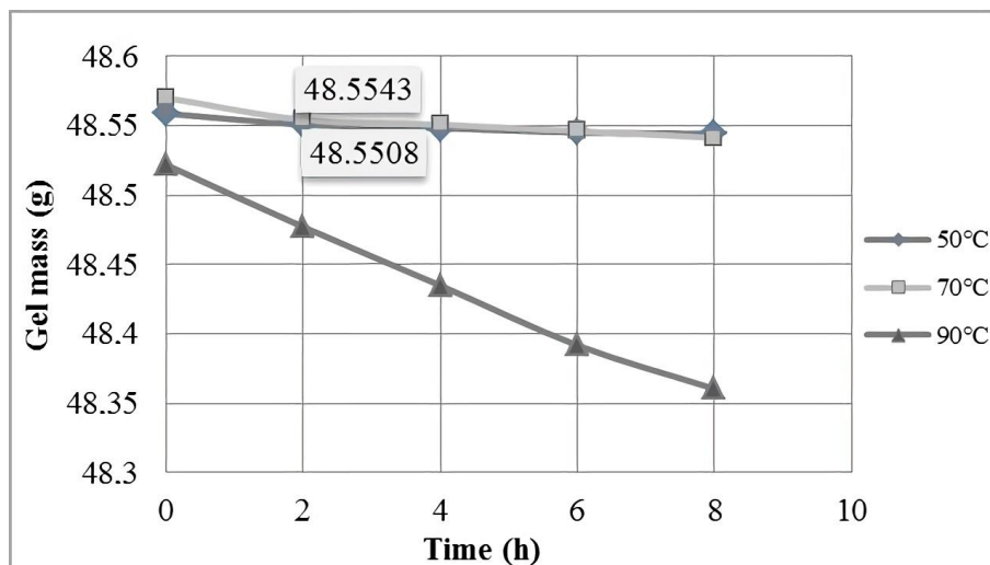
Figure 1. Linseed gel thermal stability behavior
