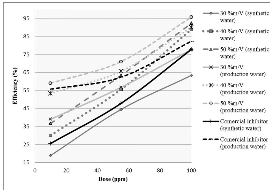
Figure 6. Experimental linseed-based inhibitors efficiency behaviors, respect to reference commercial product
