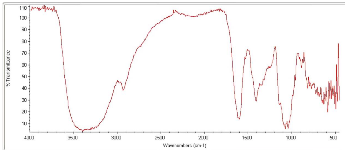
Figure 3. Infrared (IR) spectrum of linseed gel sample
