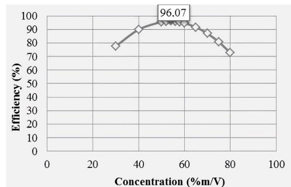
Figure 5. Graphical representation of polynomial regression for concentrations greater than 50% m/V at 100 ppm dose in production water
