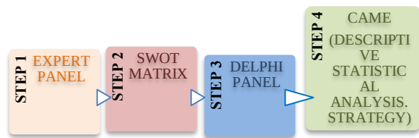
Figure 2. Methodological progress
