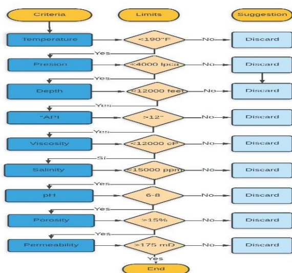
Figure 2. Flowchart representing the criteria for applying the MEOR process in the wells of Pilon Field belonging to the Morichal District.
