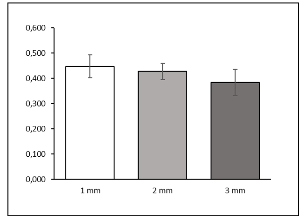
Figure 4. Effective strain means and standard deviation for groove width variations
