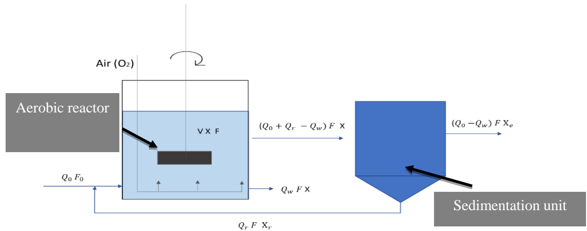
Figure 1. Schematic representation of the aerobic system used during the experimentation (check the nomenclature part).
