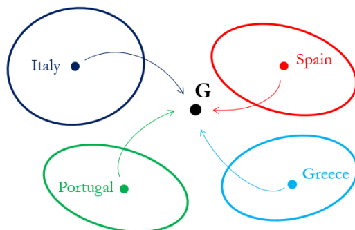
Figure 1. Recentring of point clouds in Conditional Multiple Correspondence Analysis
