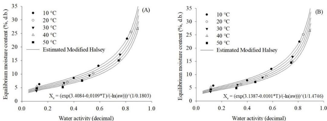
Figure 3. Observed and estimated values using the Modified Halsey model for the equilibrium moisture content obtained through desorption (A) and adsorption (B) of soybean grains at all evaluated temperatures.
