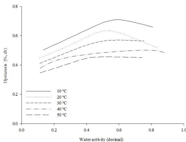
Figure 5. Effect of temperature and relative humidity on the hysteresis phenomenon in soybean grains, estimated by the Modified Halsey model.
