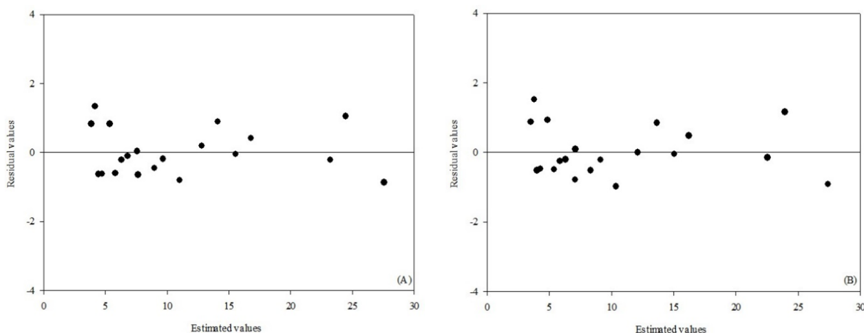
Figure 2. Random residual distribution of the Modified Halsey model for desorption (A) and adsorption (B) of soybean grains.
