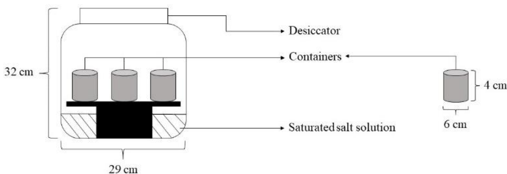
Figure 1. Schematic drawing of the samples and saturated salt solutions inside the hermetic desiccators used in the experiment.
