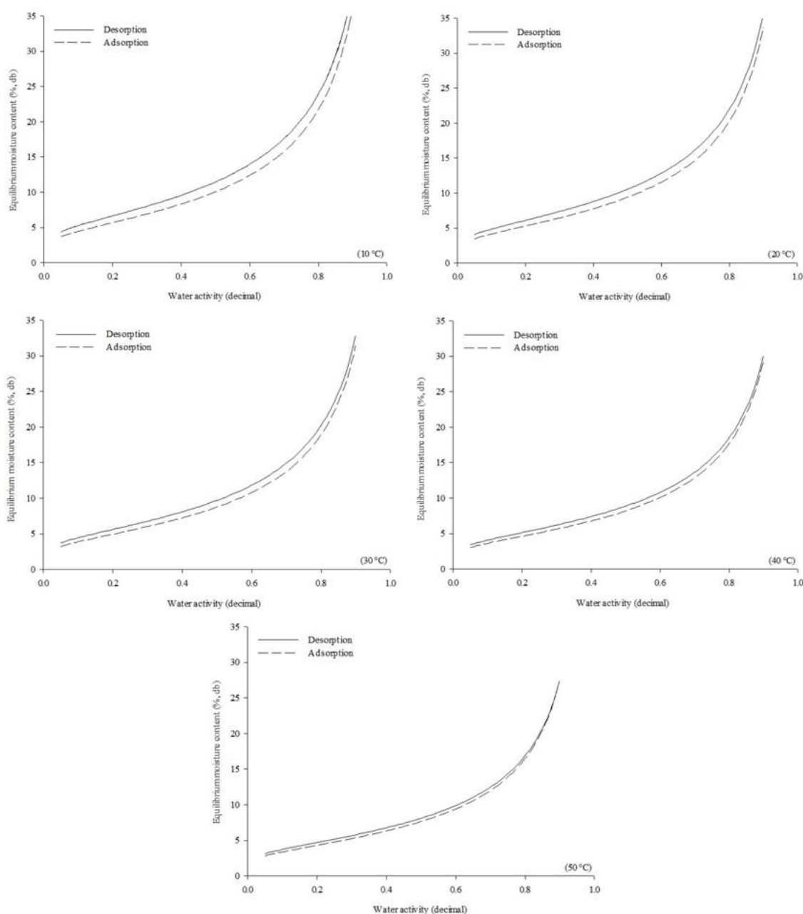
Figure 4. Desorption and adsorption isotherms of soybean grains estimated by the Modified Halsey model for all evaluated temperatures.
