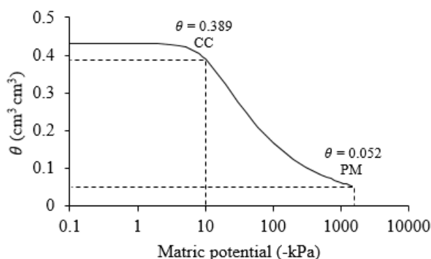
Figure 1. Soil water retention curve fitted according to the Van Genuchten model.
