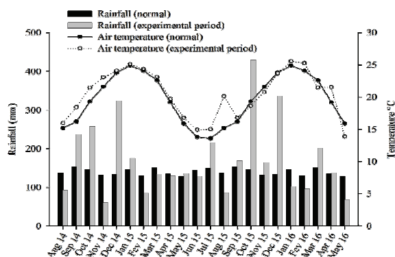
Figure 1. Climatological normals and values recorded in the experimental period for average temperature and monthly cumulative rainfall. Santa Maria, State of Rio Grande do Sul, 2014-2016.
