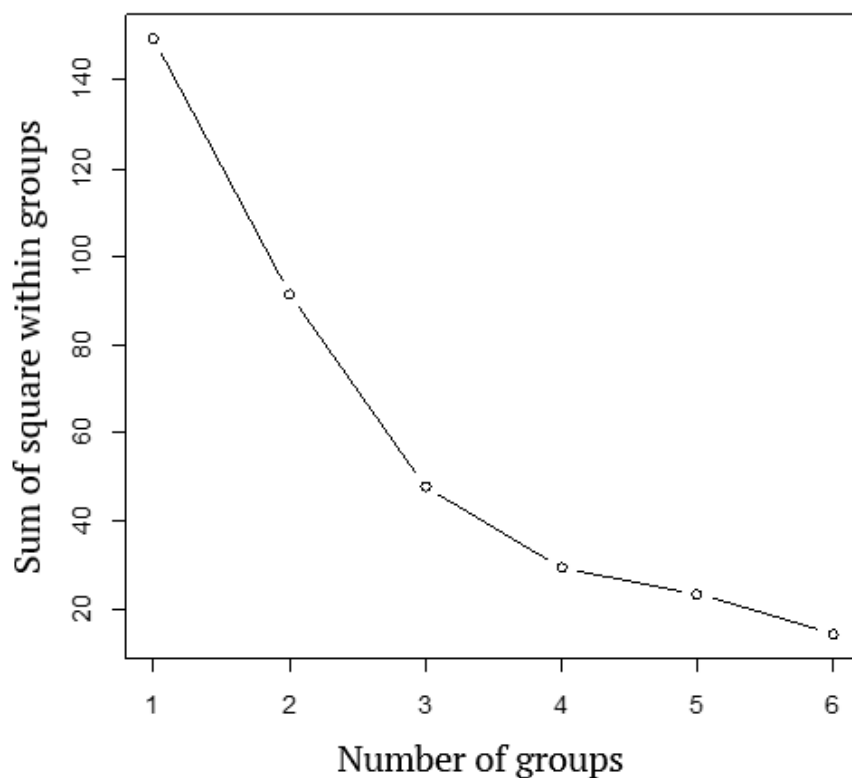
FIGURE 5. Sum of squares within the groups for different groups, using the ‘K-means’ method for the data of plate cisterns in the Pajeú, state Pernambuco. Number of groups
