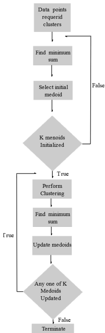
FIGURE 3. Sequential flowchart of the PAM algorithm.
