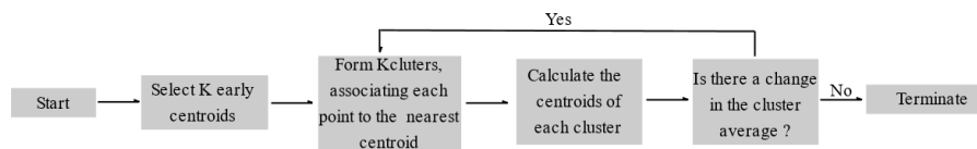
FIGURE 2. Algorithm ‘K-means’.
