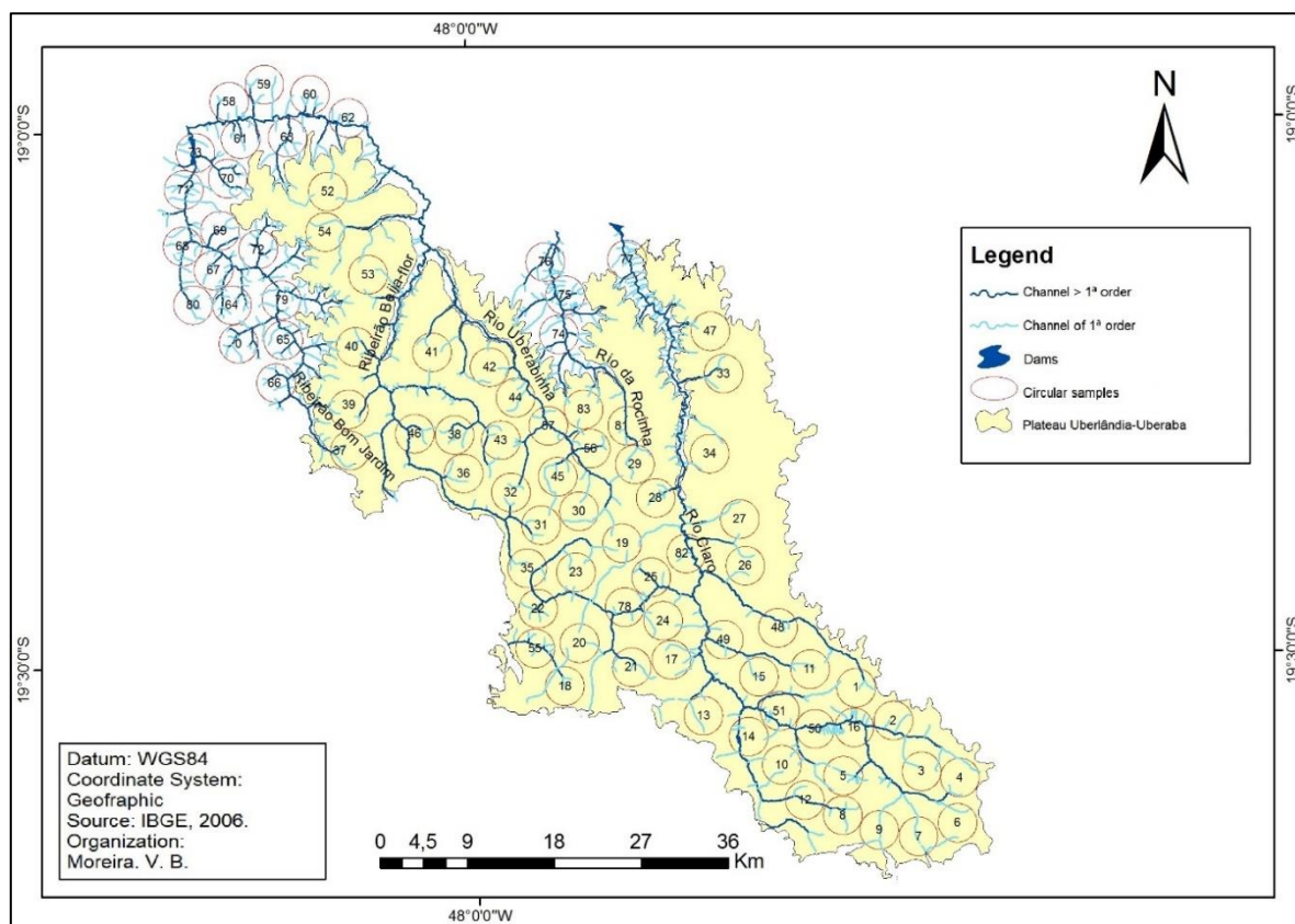
Figure 2 – Sampling of Uberlândia-Uberaba plateau and surrounding areas drainage network.
