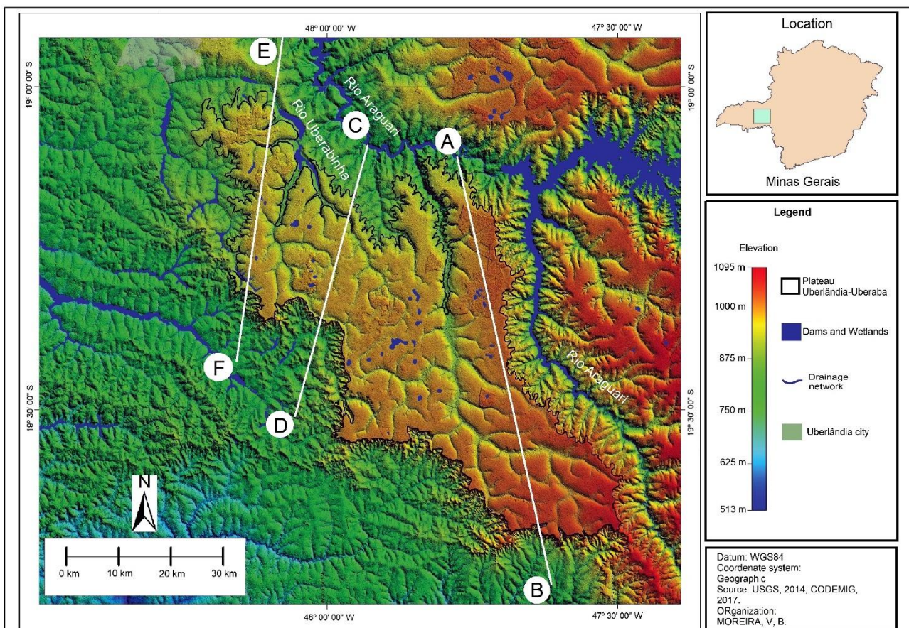
Figure 3 – Transects and regional elevation of Uberlândia-Uberaba plateau.
