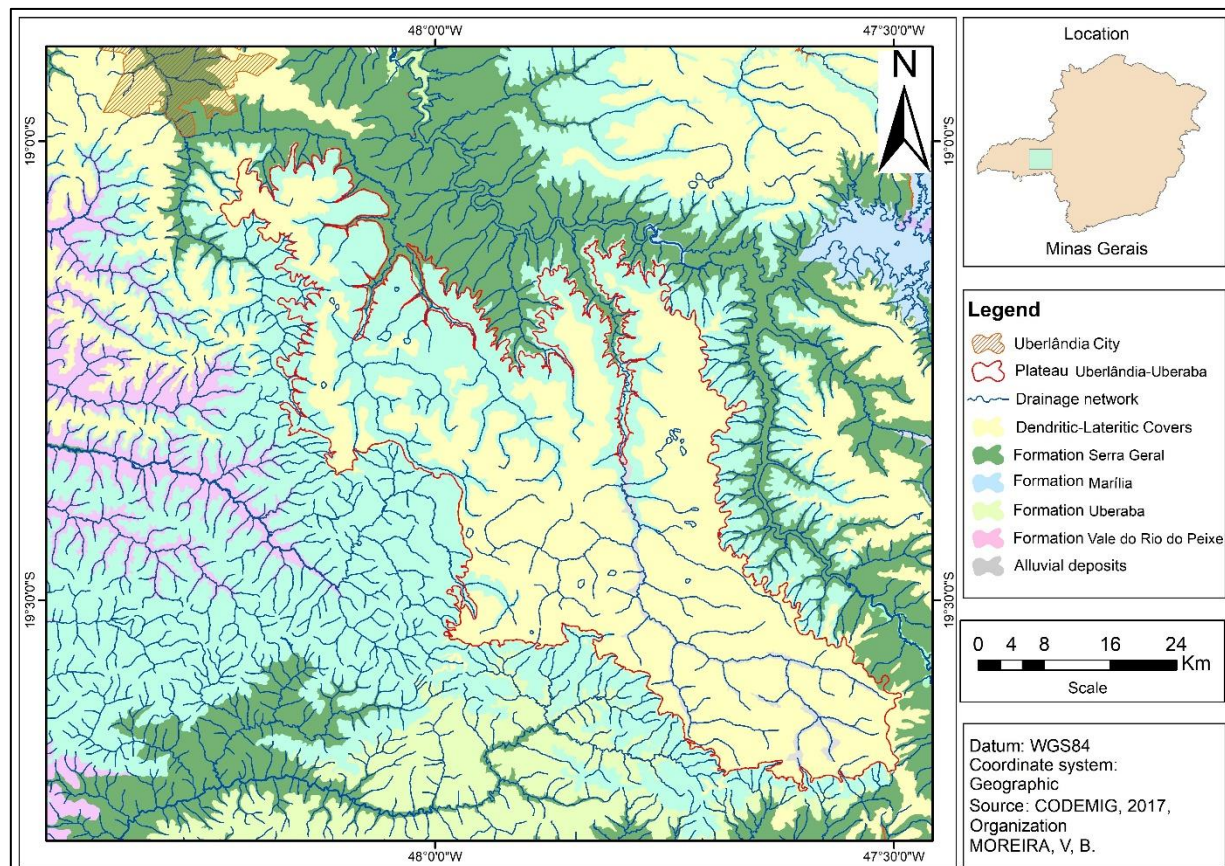
Figure 1 – Uberlândia-Uberaba plateau and surroundings litostratigraphic units.
