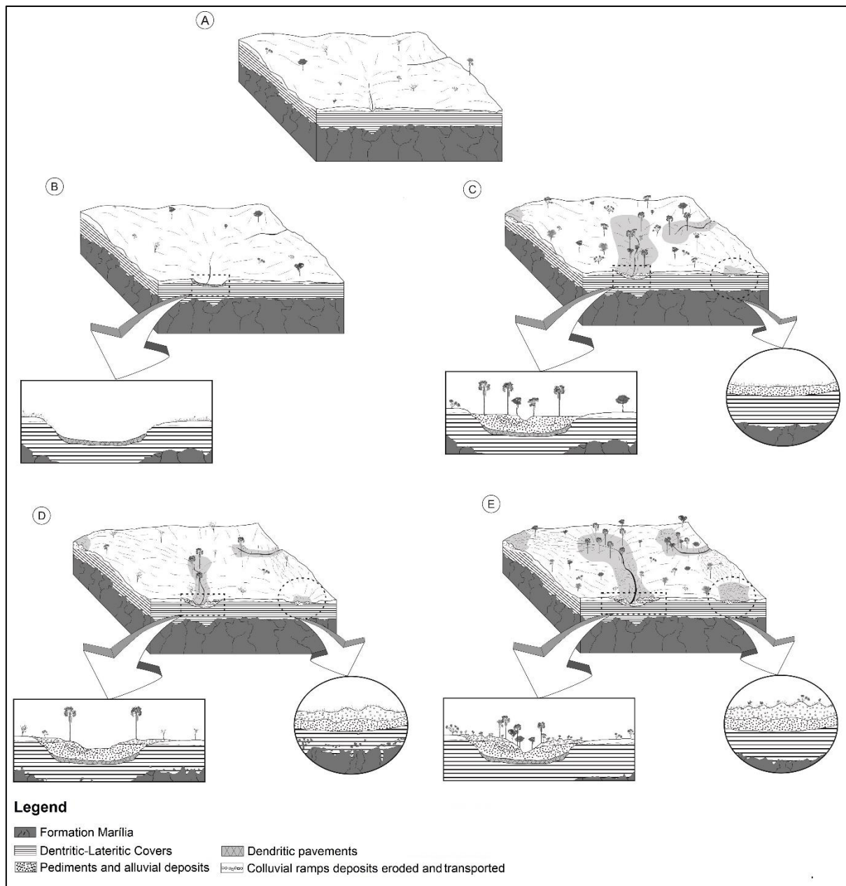
Figure 5 – Possible Uberlândia-Uberaba plateau Holocene evolutionary scenarios.
