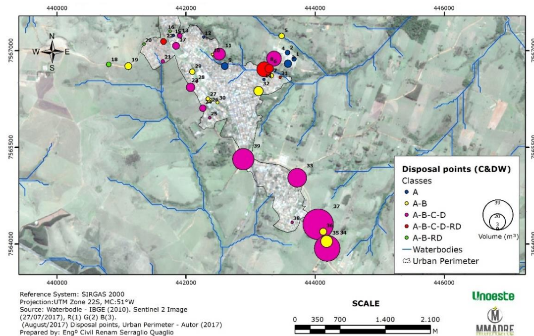
Figure 3: C&DW classes and volumes at collection points in Presidente Bernardes County-SP- Brazil.
