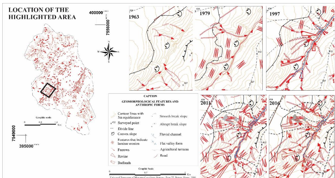
Figure 9. Evolution of erosion forms at the W subbasin, affected by the formation of badlands from 1997 onwards.
