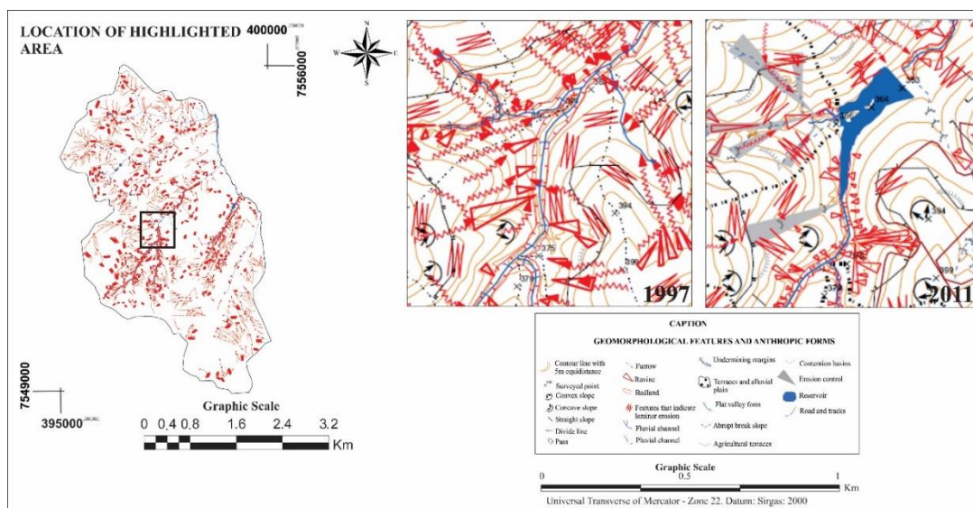
Figure 12. Changes in the pattern of formation and development of ravines after impoundment of water of badlands.
