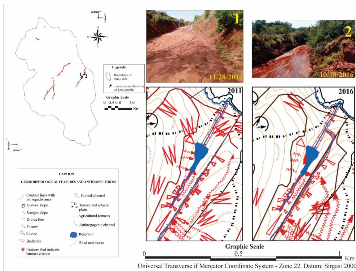
Figure 13. Influence of agricultural terraces on the flow of water in the channel of anthropogenic origin, resulting from the process of formation of badlands affecting the rural road. (1) Surface runoff at the base of badland in 2012; (2) Surface runoff at the base of badland in 2016.
