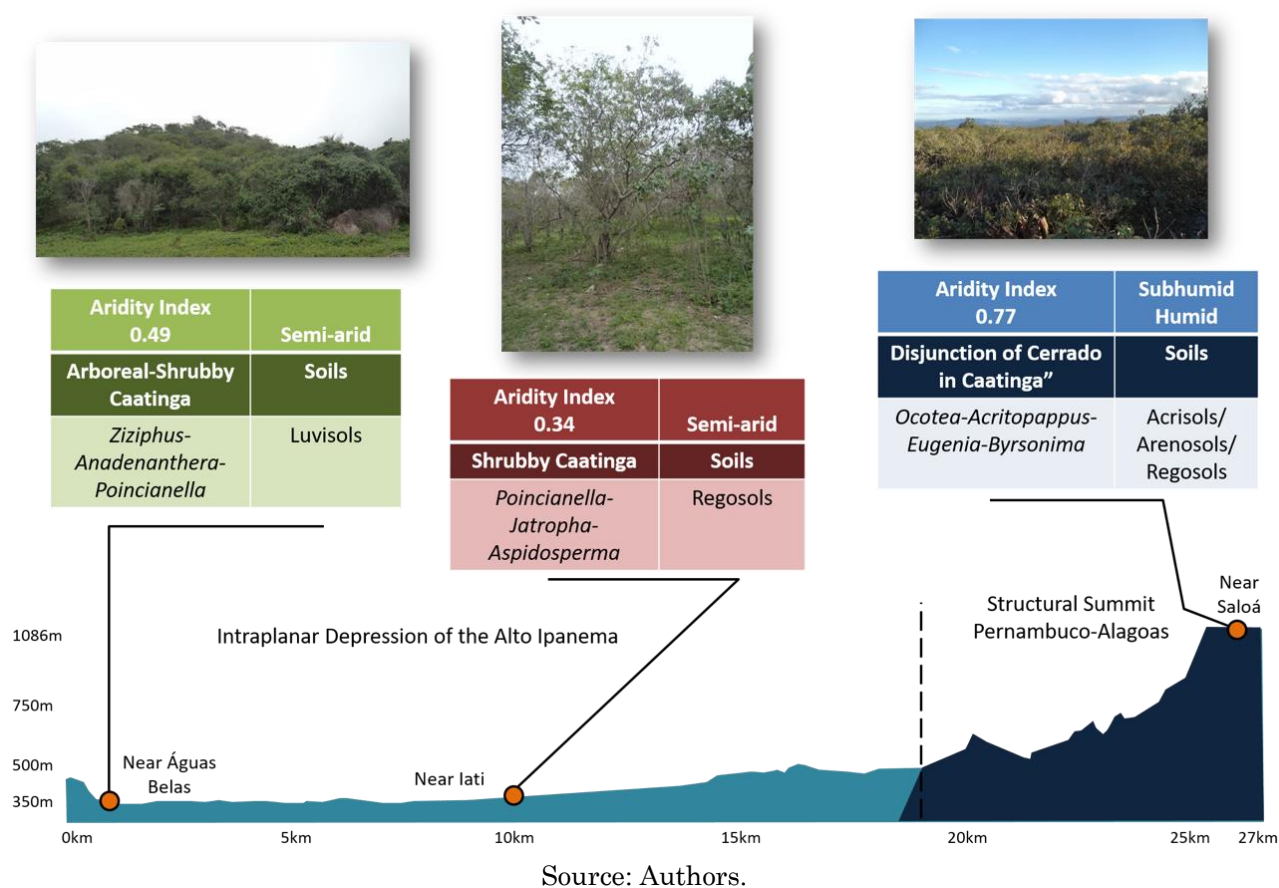
Figure 1. Landscape Profile between Águas Belas and Saloá.
