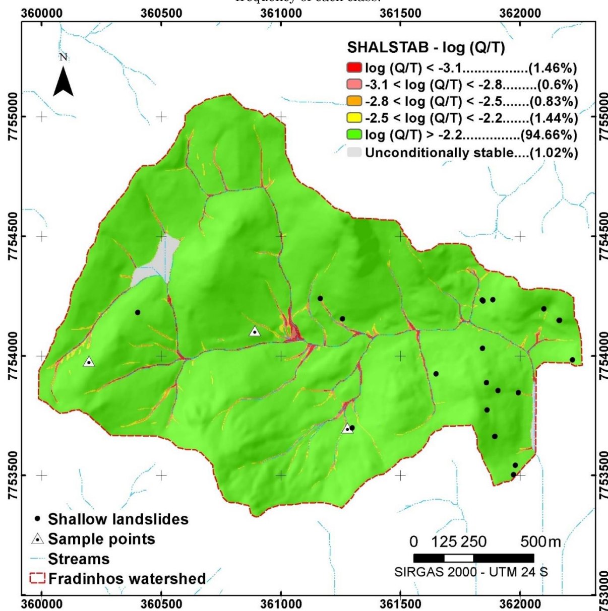
Figure 7 – Susceptibility to shallow landslides at Fradinhos watershed, with results in \log(Q/T) and frequency of each class.
