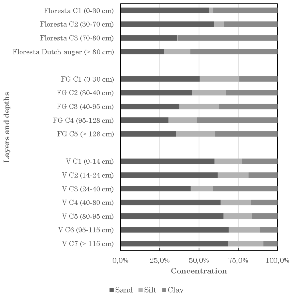
Figure 5 – Granulometric distributions from the Floresta, Fonte Grande (FG) and Varejão (V) profiles
