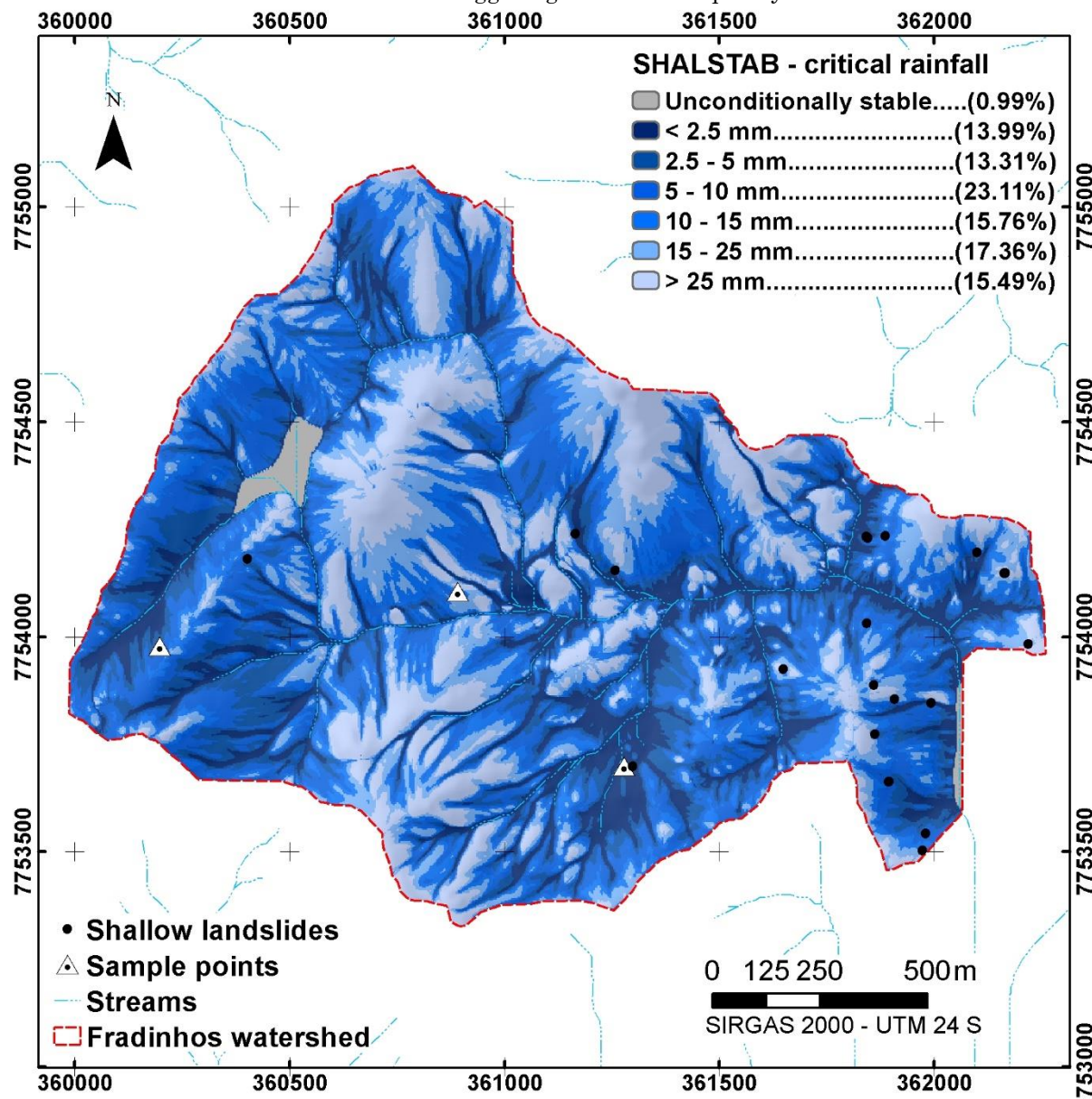
Figure 8 – Shallow landslide susceptibility at Fradinhos watershed, with results in critical rainfall needed for triggering and class frequency
