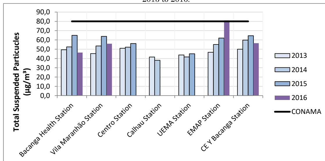
Figure 5 - Graph of the annual average of Air Quality Monitoring Stations in São Luís for TSP pollution ( \mu\text{g}/\text{m}^3 ) compared to the limits established by CONAMA resolution 3/90 in the period from 2013 to 2016.
