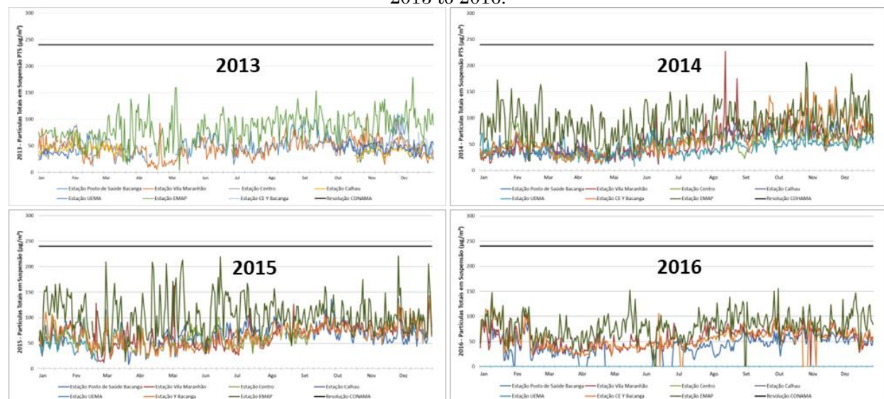
Figure 8 - Graphs of the daily averages of all Air Quality Monitoring Stations in São Luís for IP pollution ( <10\mu\text{m}^3 ) compared to the limits established by CONAMA Resolution 3/90 in the years 2013 to 2016.
