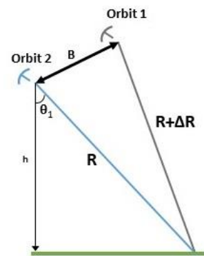
Figure 1. InSAR geometry scheme obtained from two orbits
