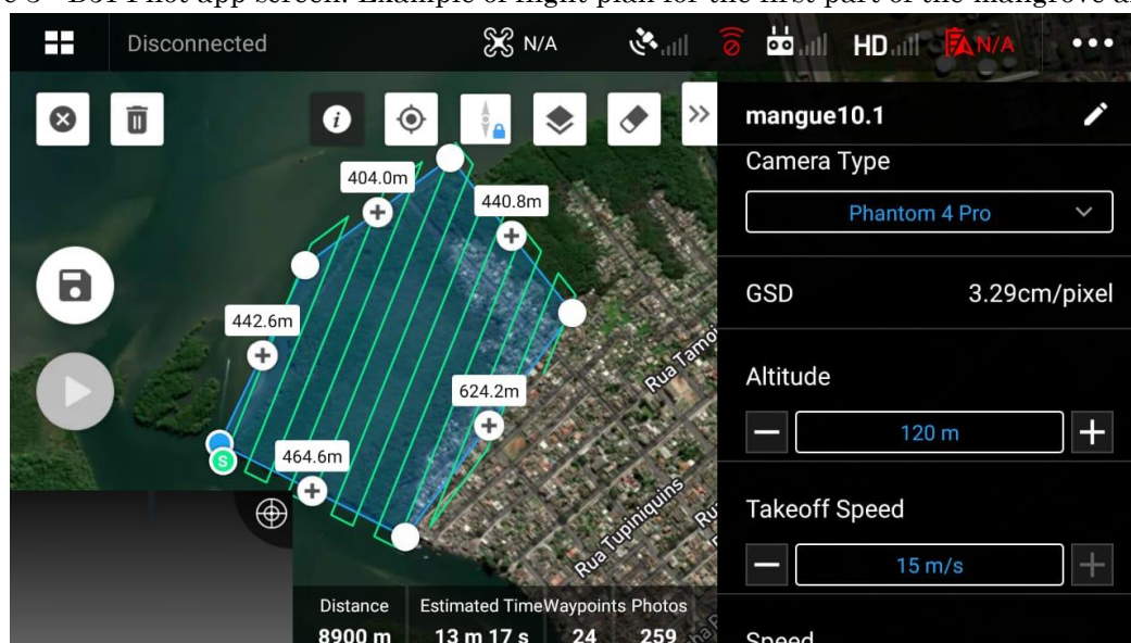
Figure 3 - DJI Pilot app screen. Example of flight plan for the first part of the mangrove area 04.
