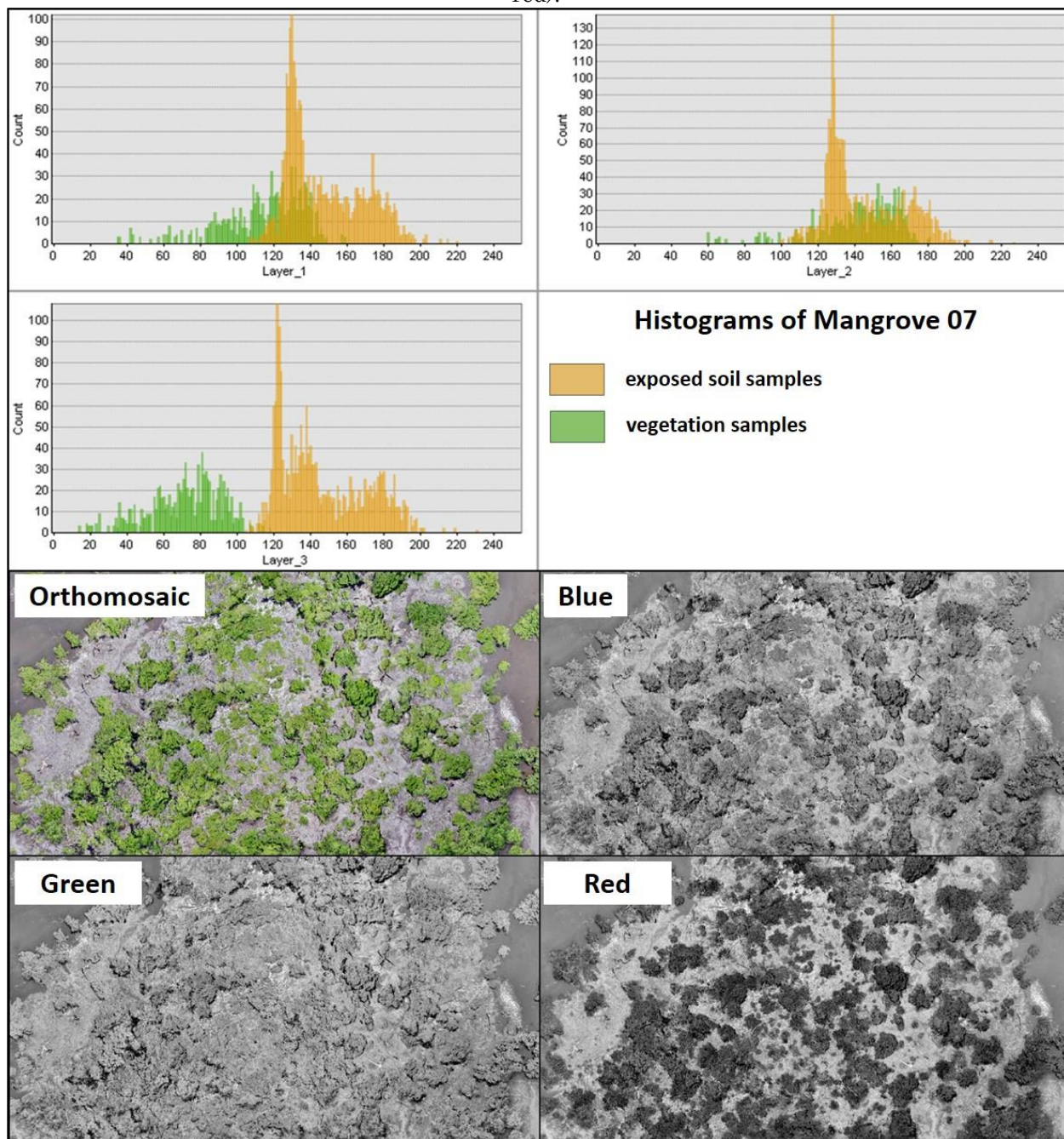
Figure 4 - Example of histograms of samples collected for classification of mangrove orthomosaic 07. Below the histograms, individual visualization of each band (Layer_1: blue; Layer_2: green; Layer_3: red).
