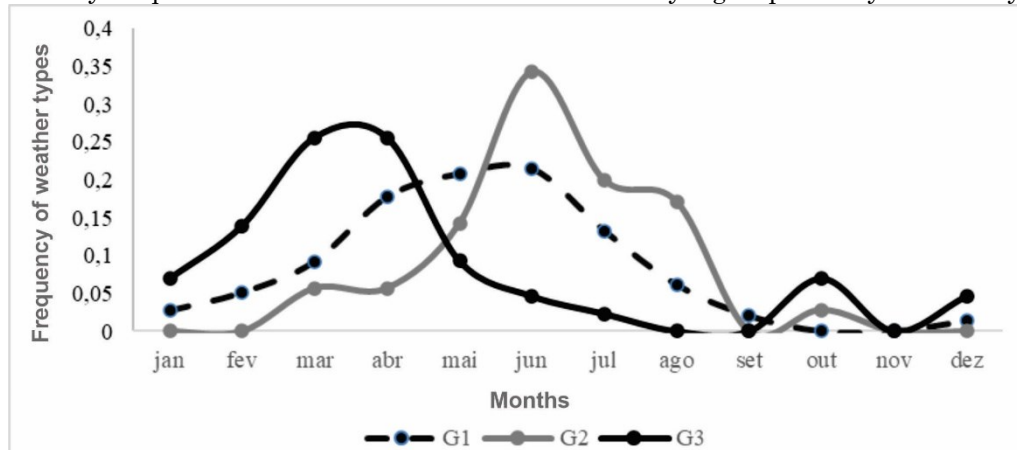
Figure 5 - Monthly frequencies of occurrence of intense rainfall by a group of daily weather types.
