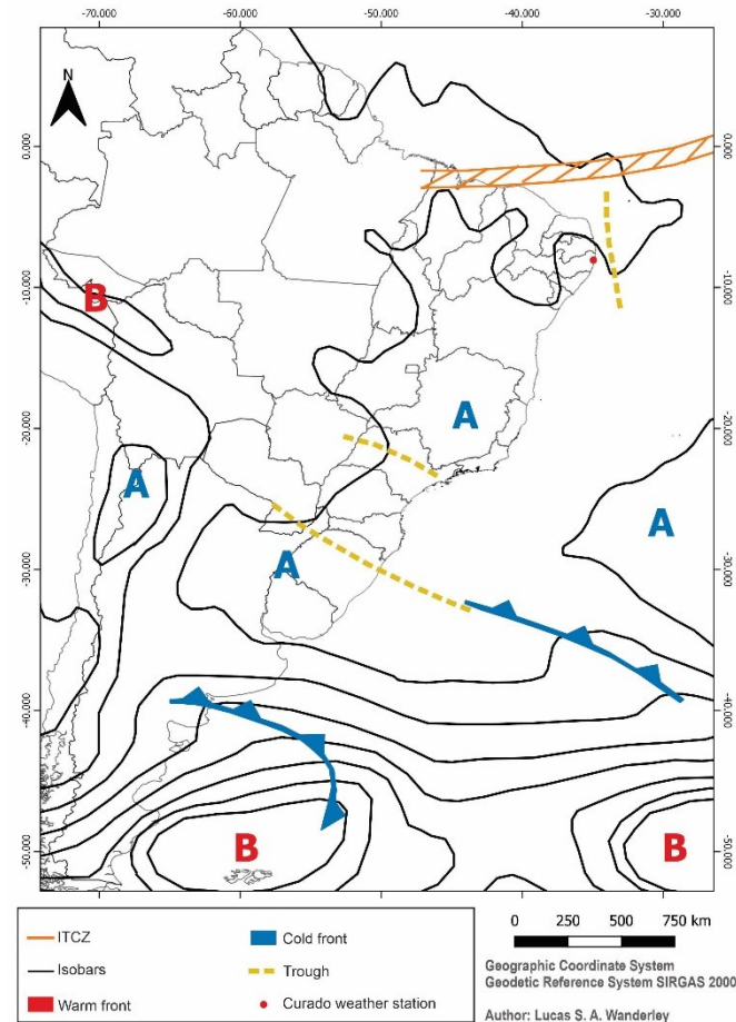
Figure 9 - Synoptic chart at 0h UTC on 04/06/2009 for part of South America and the Atlantic Ocean.
