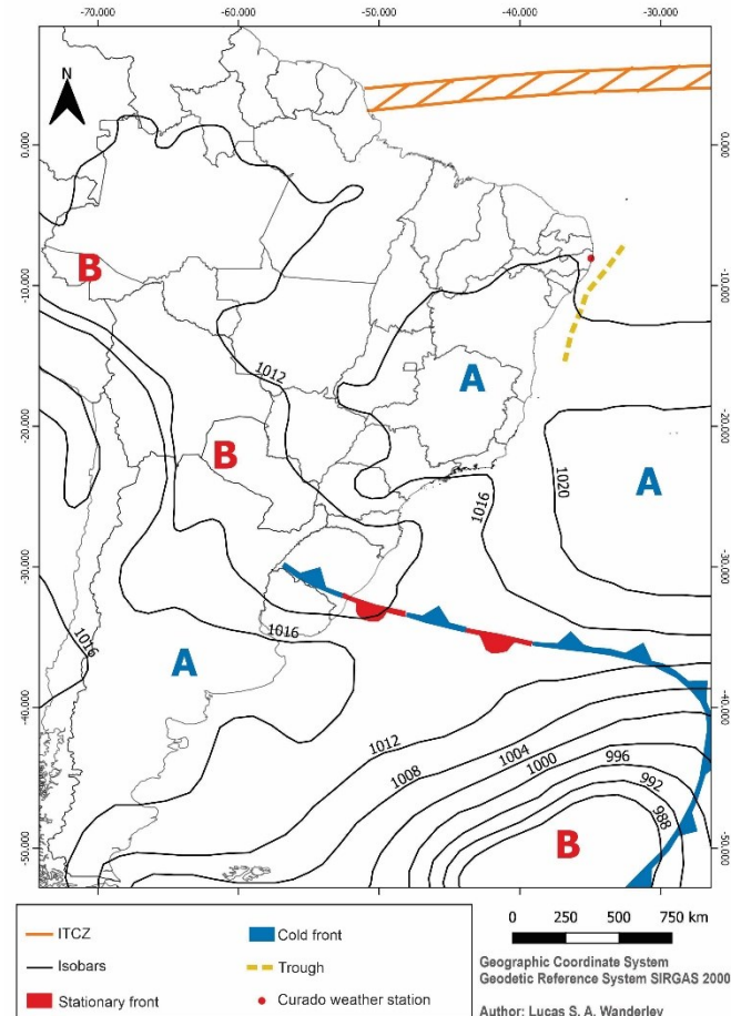
Figure 6 – Synoptic chart at 0h UTC on 06/17/2010 for part of South America and the Atlantic Ocean.
