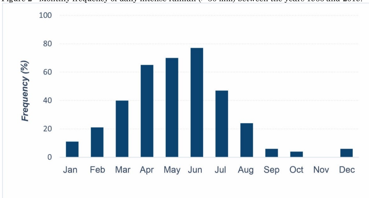
Figure 2 - Monthly frequency of daily intense rainfall (> 50 mm) between the years 1966 and 2019.
