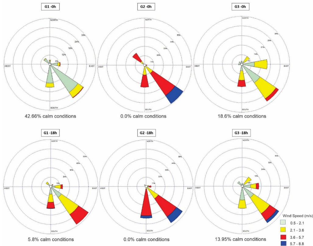
Figure 4 - Wind roses referring to the grouped weather types for the hours of 0h and 18h UTC.
