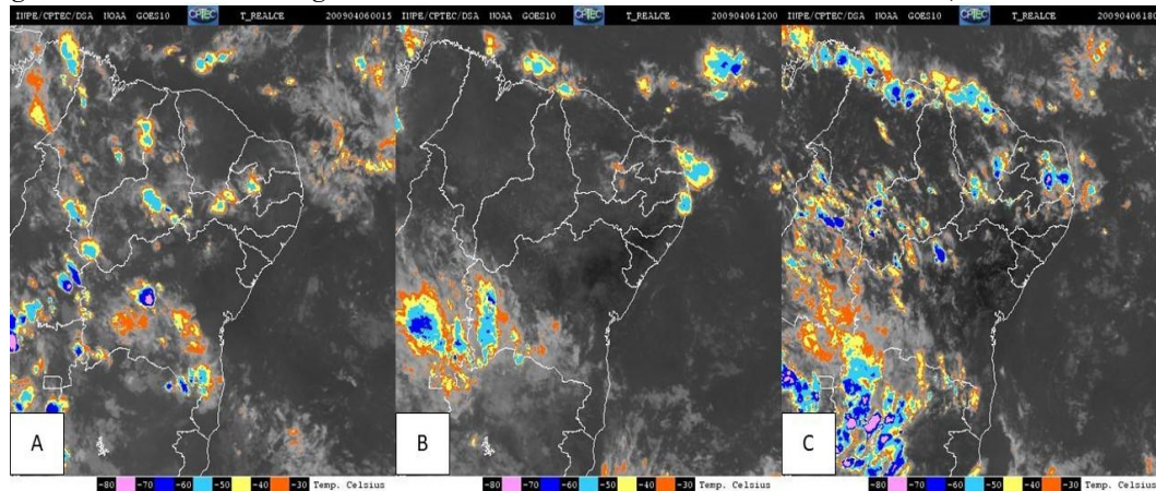
Figure 10 - Satellite images of the enhanced channel for 04/06/2009 at 0, 12 and 18h UTC.
