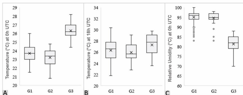
Figure 3 - Boxplot charts for temperatures at 0h (A) and 18h (B), and relative humidity at 0h (C) for the grouped daily weather types.
