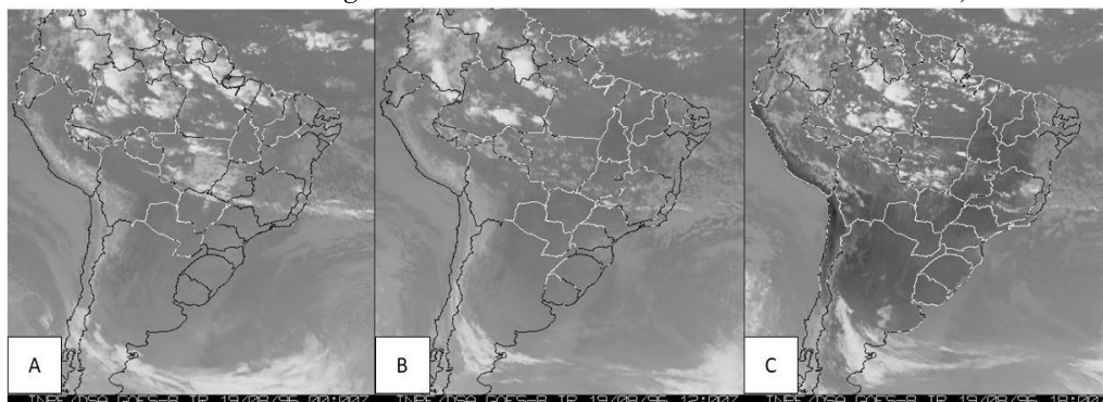
Figure 8 - GOES-8 satellite images of the infrared channel for 08/19/1996 at 0, 12 and 18h UTC.
