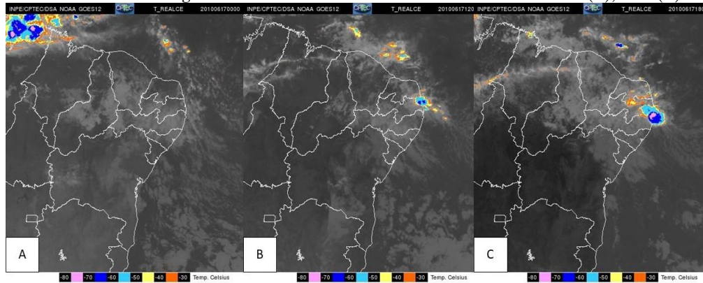
Figure 7 - GOES satellite images in the enhanced channel for 06/17/2010 at 0h (A), 12h (B) and 18h (C).
