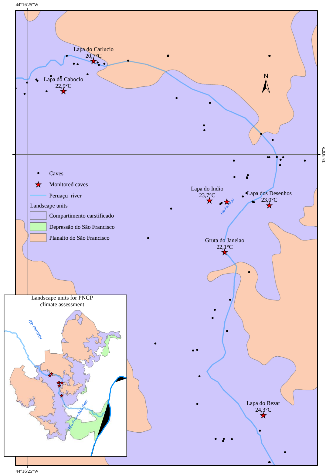
Figure 4 - Landscape units used for the study of the climate in the PNCP (Serafini-Júnior, 2005), with emphasis on the disposition of the monitored caves along the Peruaçu River Canyon and the respective average temperatures measured at each entrance.
