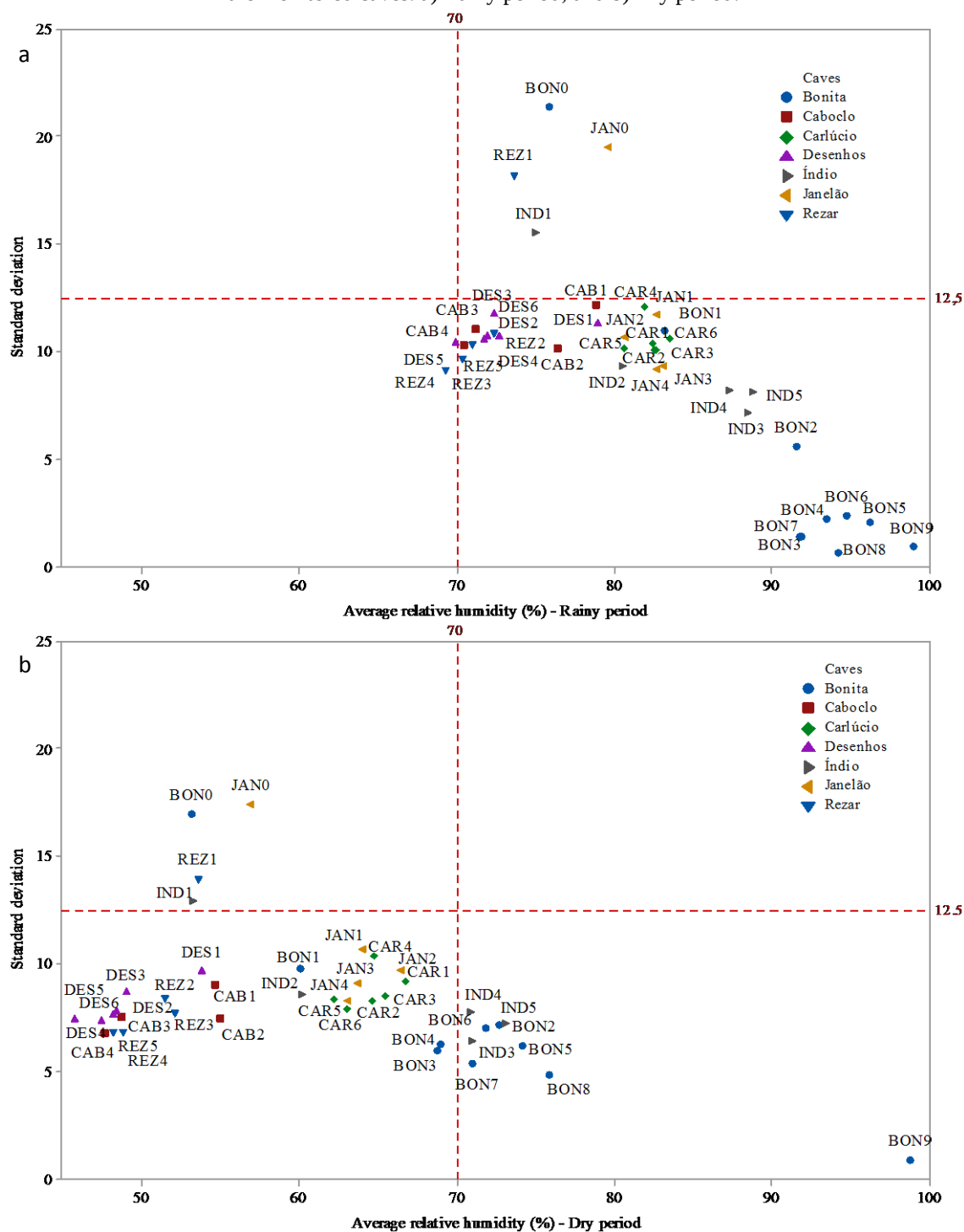
Figure 9 – Analysis of standard deviation according to relative humidity measurements for the data collected from the monitored caves. a) Rainy period; and b) Dry period.
