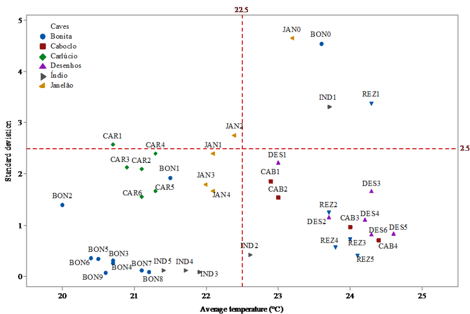
Figure 5 – Analysis of the standard deviation according to average temperatures for the data collected in the monitored caves.
