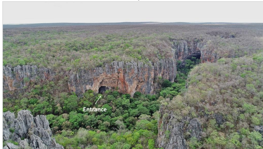
Figure 6 - Aerial view of the entrance to Lapa do Carlúcio highlighting the riparian forest of the Peruaçu River at the bottom of the canyon.
