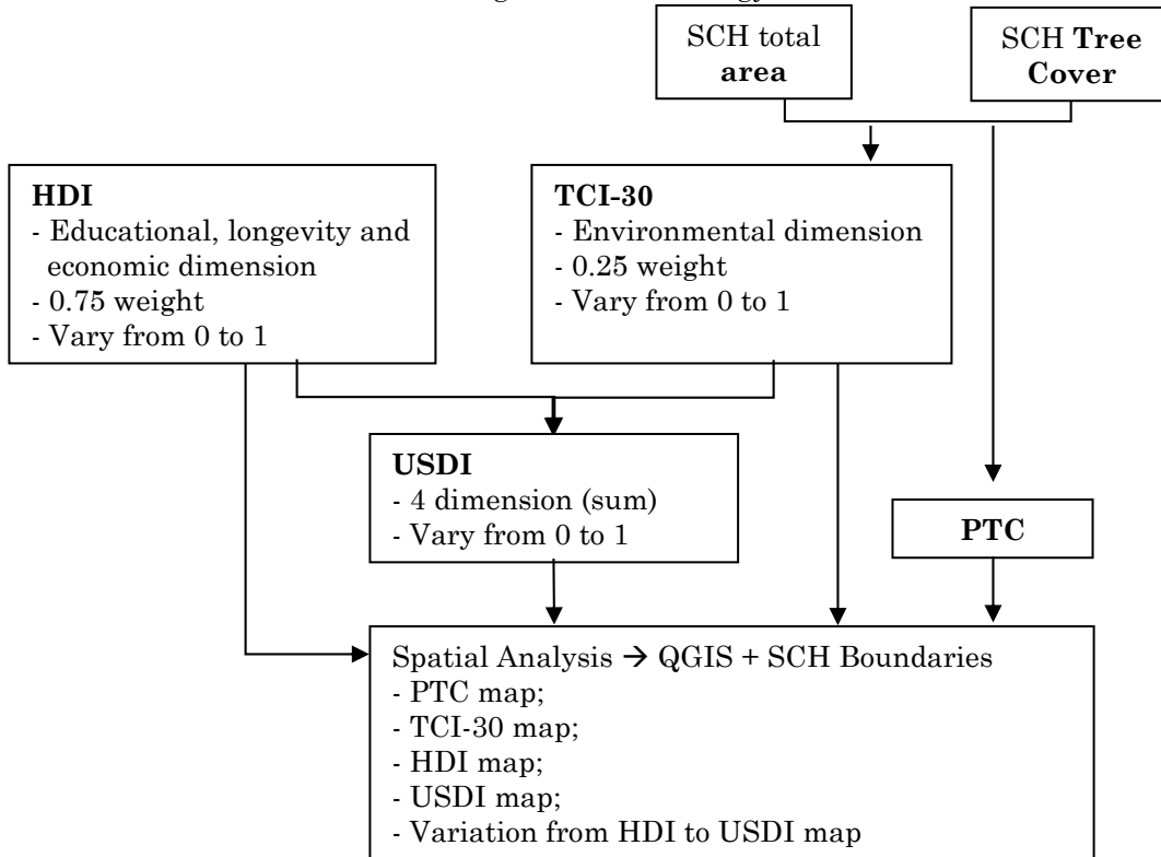
Figure 3 -Methodology flowchart.
