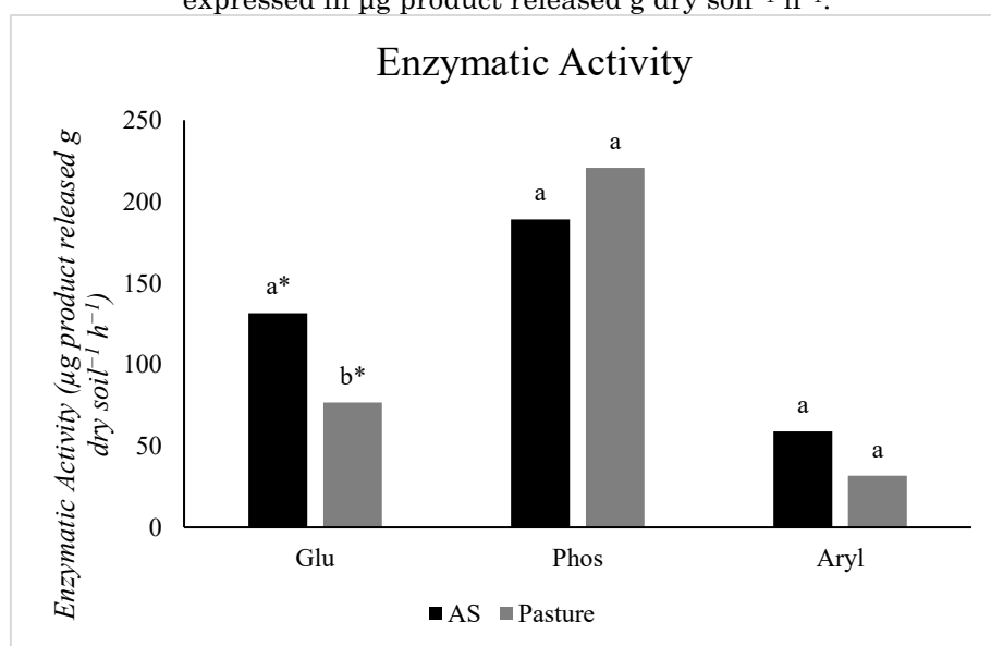
Figure 4 - Concentration of the enzymes \beta -glucosidase, phosphatase and Arylsulfatase in the management of Agroecological Systems and Pasture. The values of the enzymatic activities were expressed in \mu\text{g product released g dry soil}^{-1} \text{ h}^{-1} .
