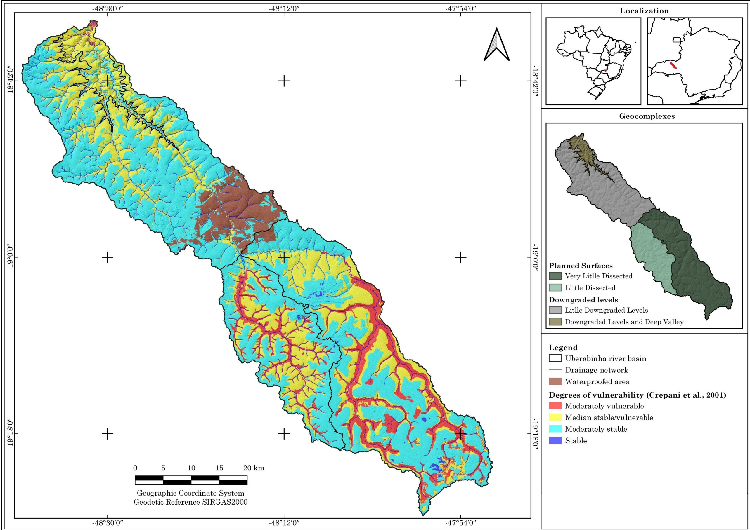
Figure 6 – Vulnerability to soil loss in the Uberabinha river basin.
