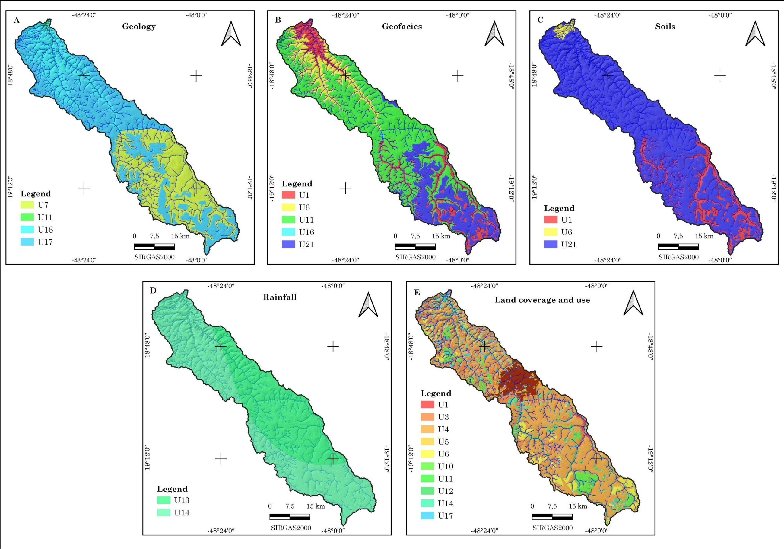
Figure 5 – Vulnerability units of the Uberabinha river basin. A) Geology; B) Geofacies; C) Soils; D) Rainfall; E) Land cover and use.
