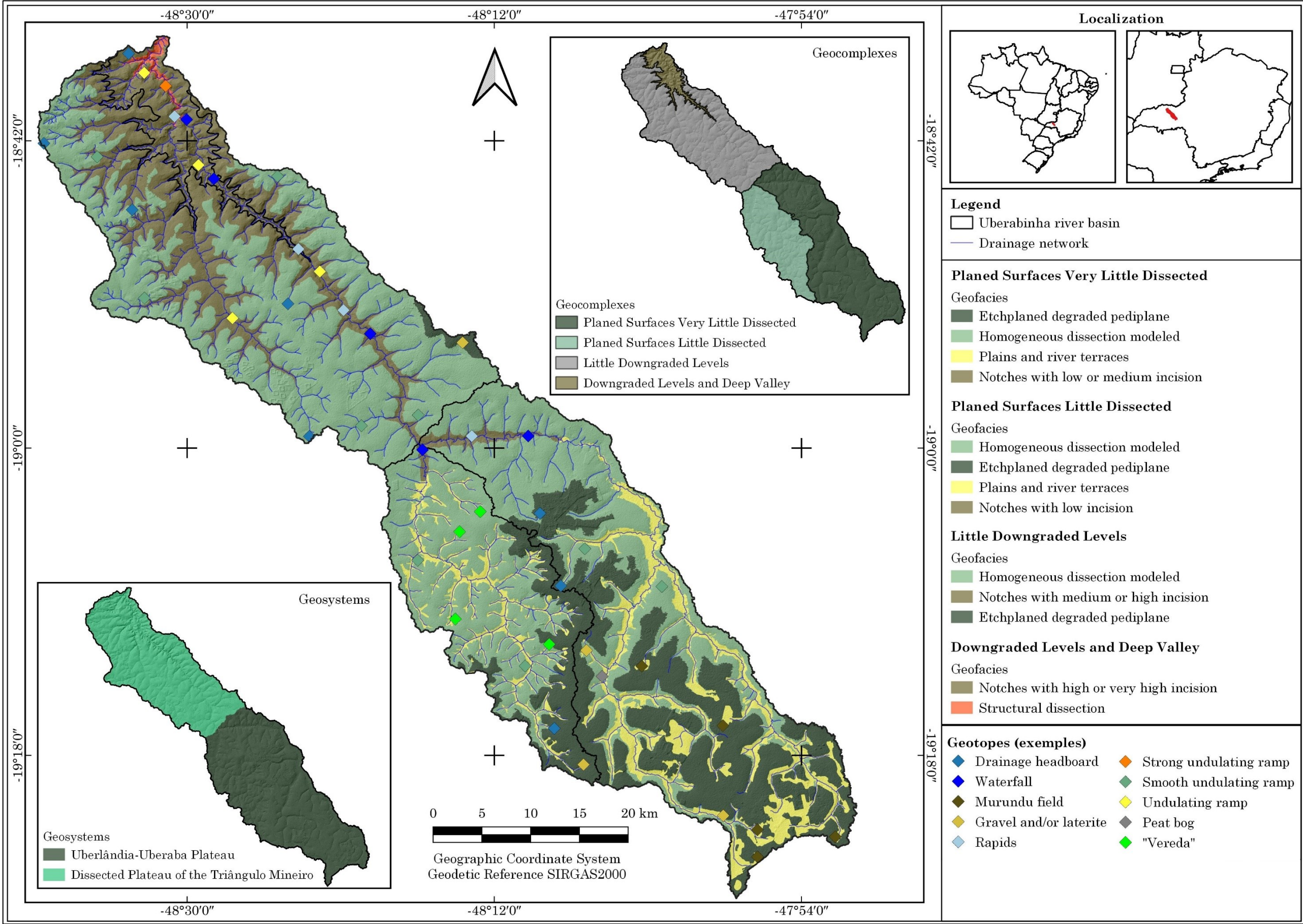
Figure 3 – Subdivision of geosystems in the Uberabinha river basin.
