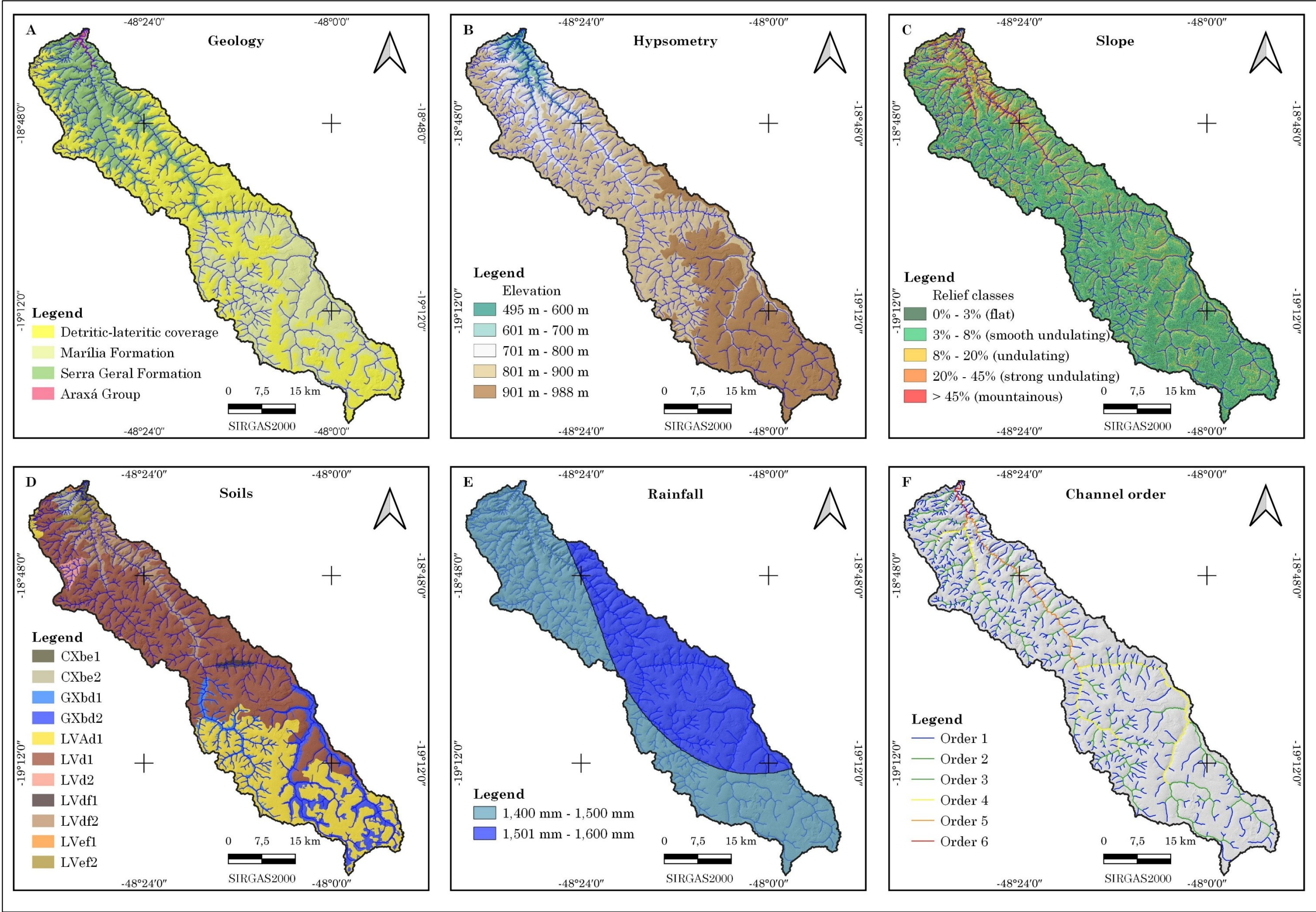
Figure 2 – Physiographic components of the Uberabinha river basin. A) Geology; B) Hypsometry; C) Declivity; D) Soils; E) Rainfall; F) Order of channels.
