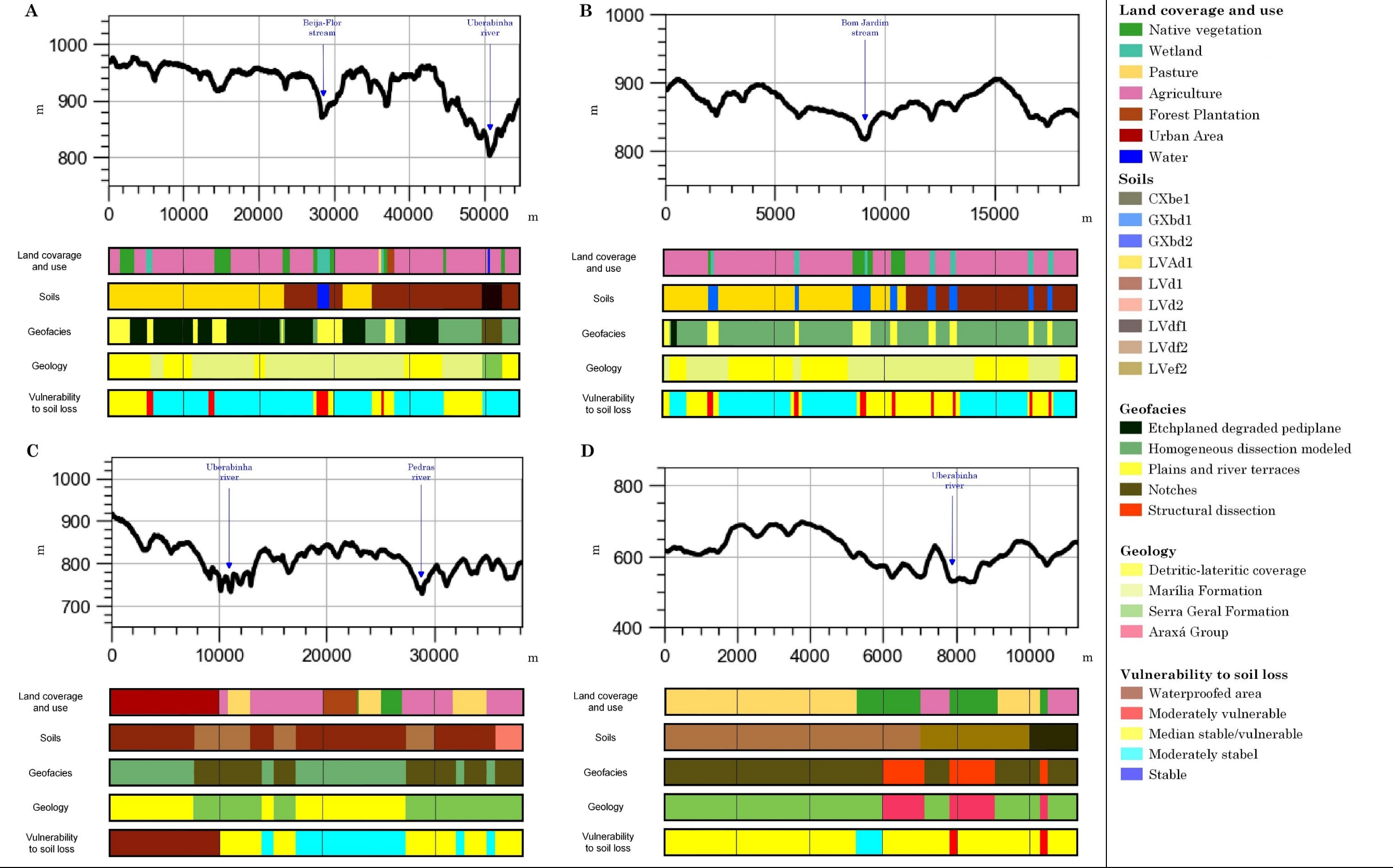
Figure 8 – Geocological profiles. A) Profile traced in the Planed Surfaces Very Little Dissected geocomplex; B) Profile traced in the Planed Surfaces Little Dissected geocomplex; C) Profile traced in the Little Downgraded Levels geocomplex; D) Profile traced in the Downgraded Levels and Deep Valley geocomplex.
