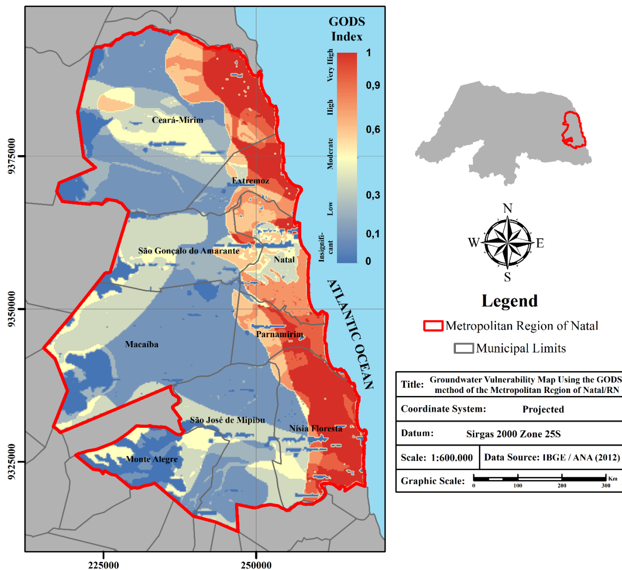
Figure 07 - Map of intrinsic vulnerability index to contamination in the aquifers of MRN
