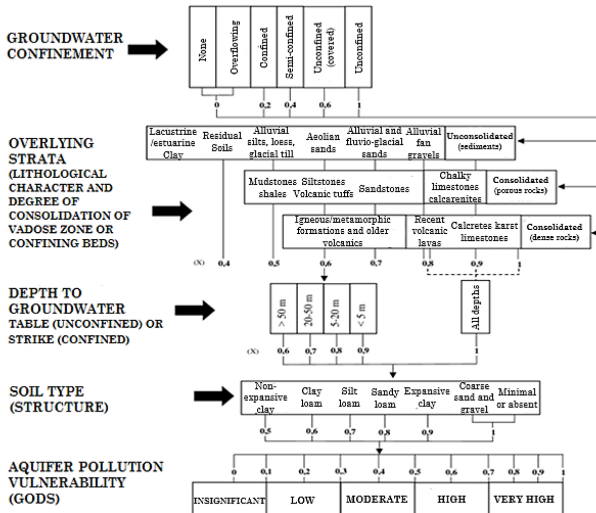
Figure 02 - GODS method for assessing aquifer contamination vulnerability.
