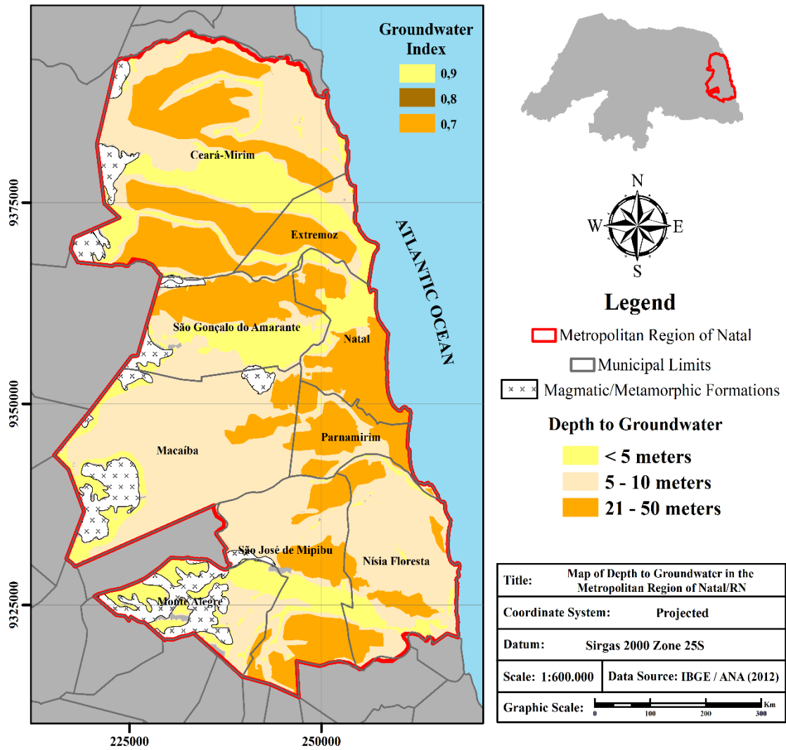
Figure 05 - Parameter D. Distance to groundwater level in the MRN aquifers.
