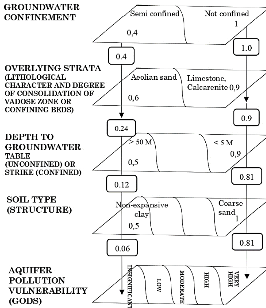
Figure 03 - Procedures adopted in the construction of the vulnerability map based on the GODS method.
