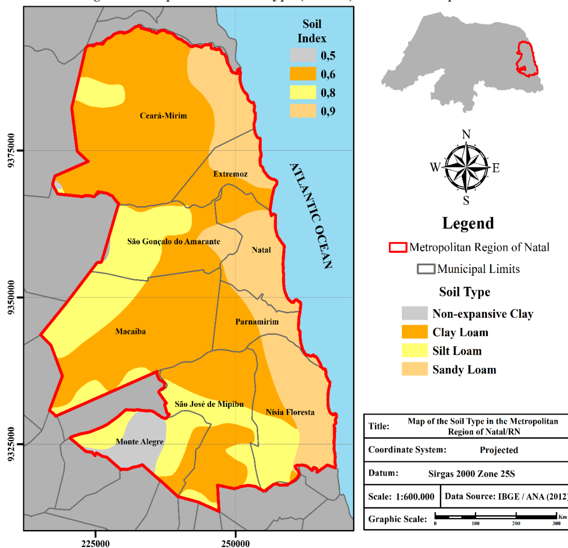
Figure 06 - S parameter. Soil type (texture) in the MRN aquifers.
