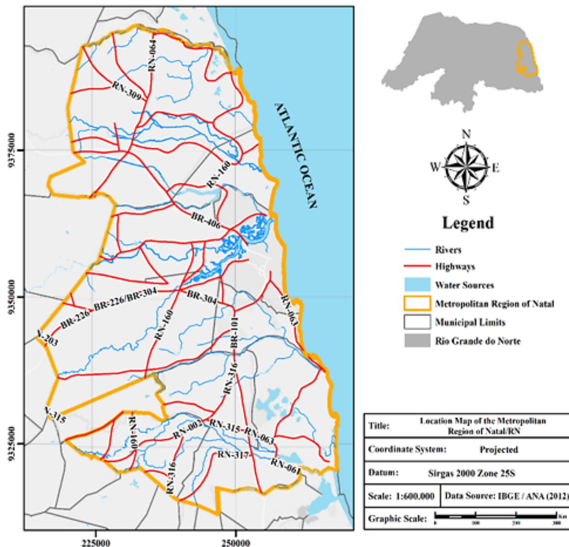
Figure 01 - Study area: Metropolitan Region of Natal (MRN).
