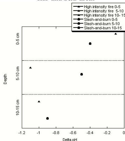
Figure 7 – Soil \Delta pH at different depths in the HIF and S&B areas
