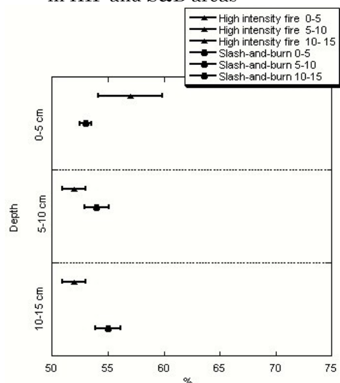
Figure 2 – Soil total porosity at different depths in HIF and S&amp;B areas
