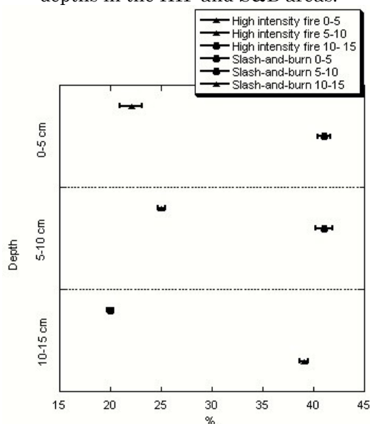
Figure 3 – Soil macroporosity at different depths in the HIF and S&amp;B areas.
