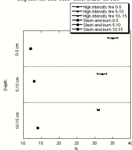
Figure 4 – Soil microporosity at different depths in the HIF and S&amp;B areas
