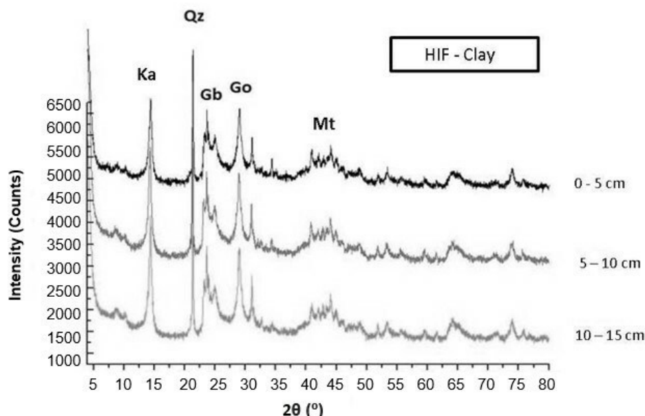
Figure 8 – Overlap of X-ray diffractograms of the clay soil fraction in the HIF area. Co K \alpha radiation (35 kV/40 mA). Ka – Kaolinite, Qz – Quartz, Gb – Gibbsite, Go – Goethite, Mt – Muscovite.
