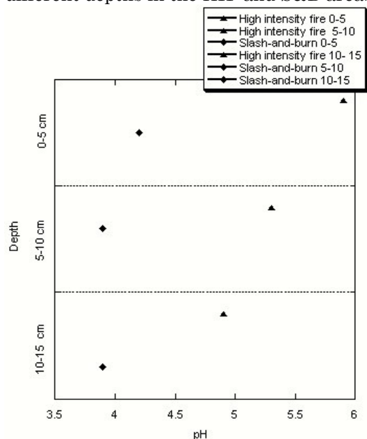
Figure 6 - Soil pH measured in KCl at different depths in the HIF and S&B areas
