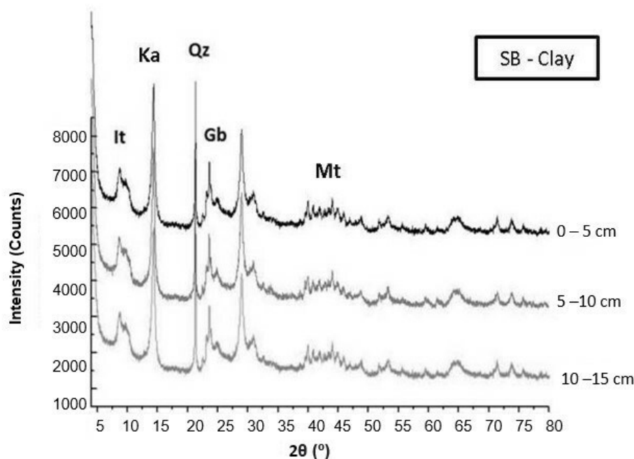
Figure 9 – Overlap of X-ray diffractograms of the clay soil fraction in the S&B area. Co K \alpha radiation. It – Illite, Ka – Kaolinite, Qz – Quartz, Gb – Gibbsite, Mt – Muscovite.
