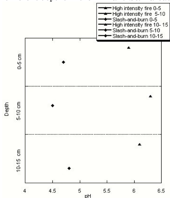
Figure 5 – Soil pH measured in water at different depths in the HIF and S&B areas
