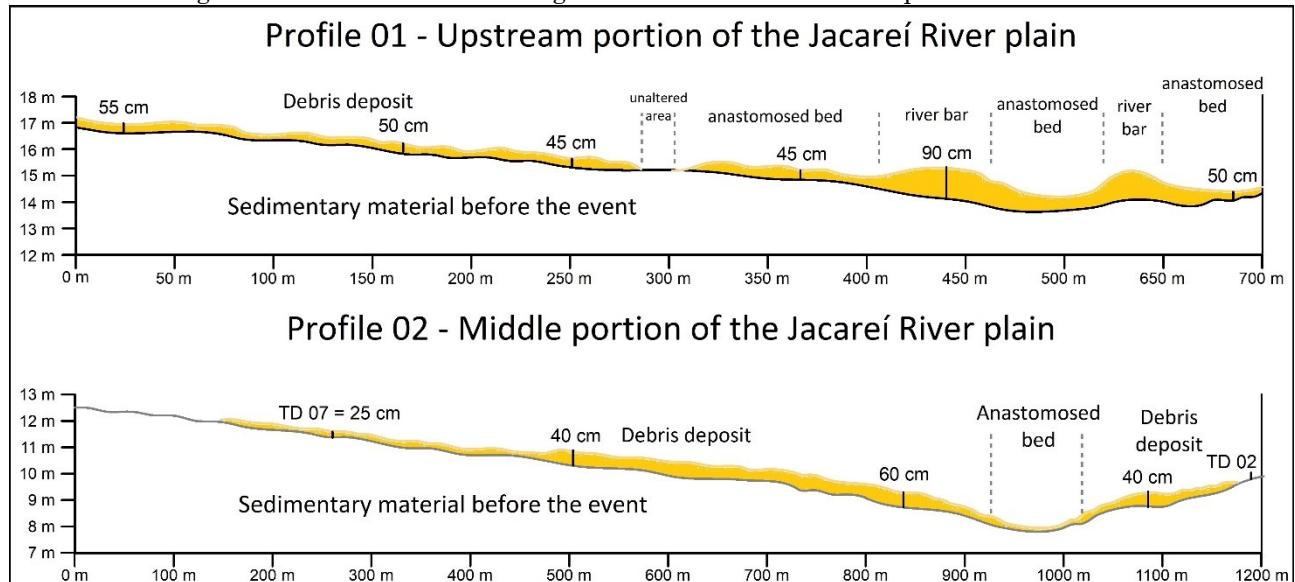
Figure 9 - Transects illustrating the vertical variation in deposit thickness.
