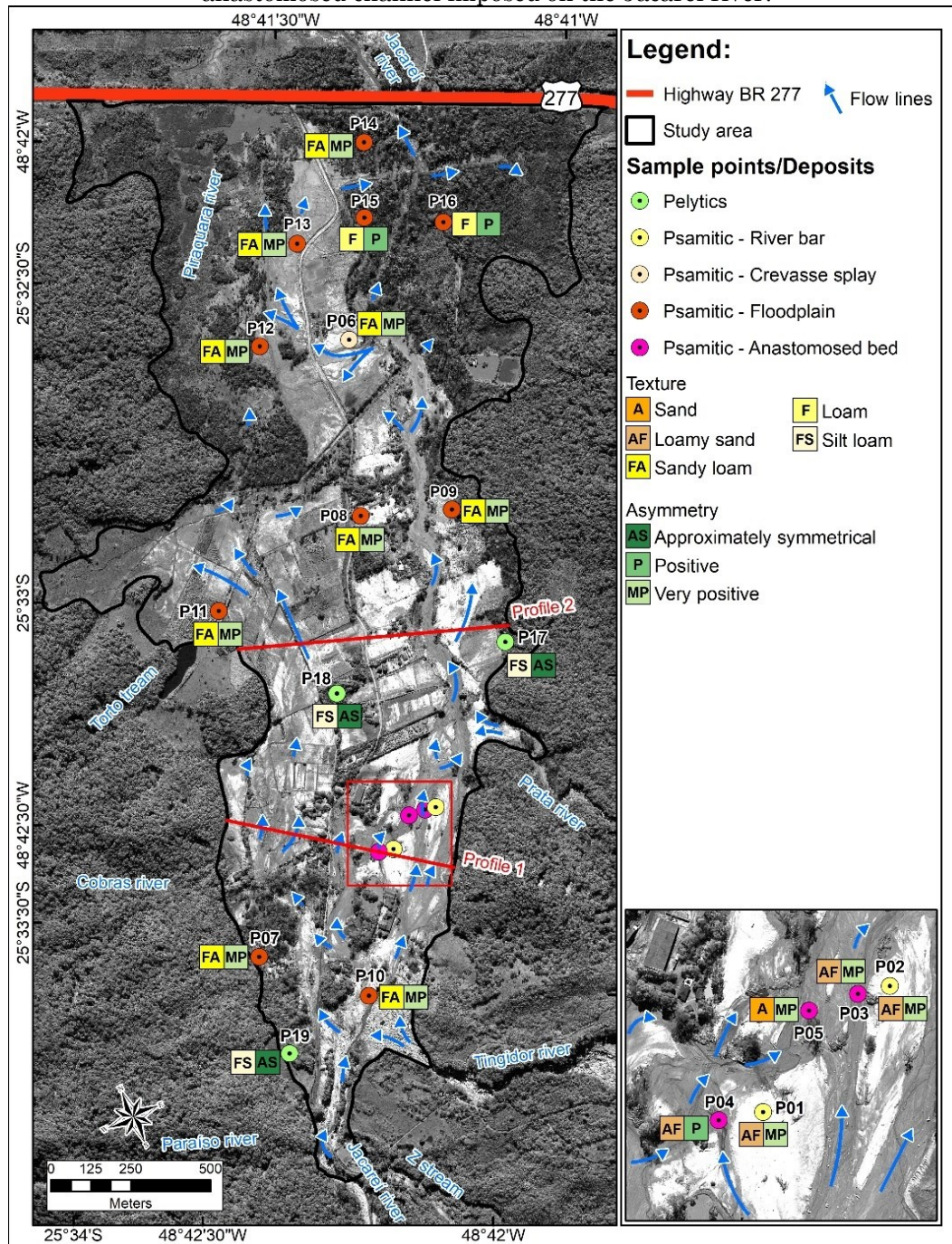
Figure 8 - Main granulometric parameters and flow lines in the alluvial plain of the Jacaréí River in 2011. Note that, after the mud flow event and the consequent of burial of the alluvial plain, it is not possible to identify the fluvial channels due to their filling. It is only possible to observe the anastomosed channel imposed on the Jacaréí river.
