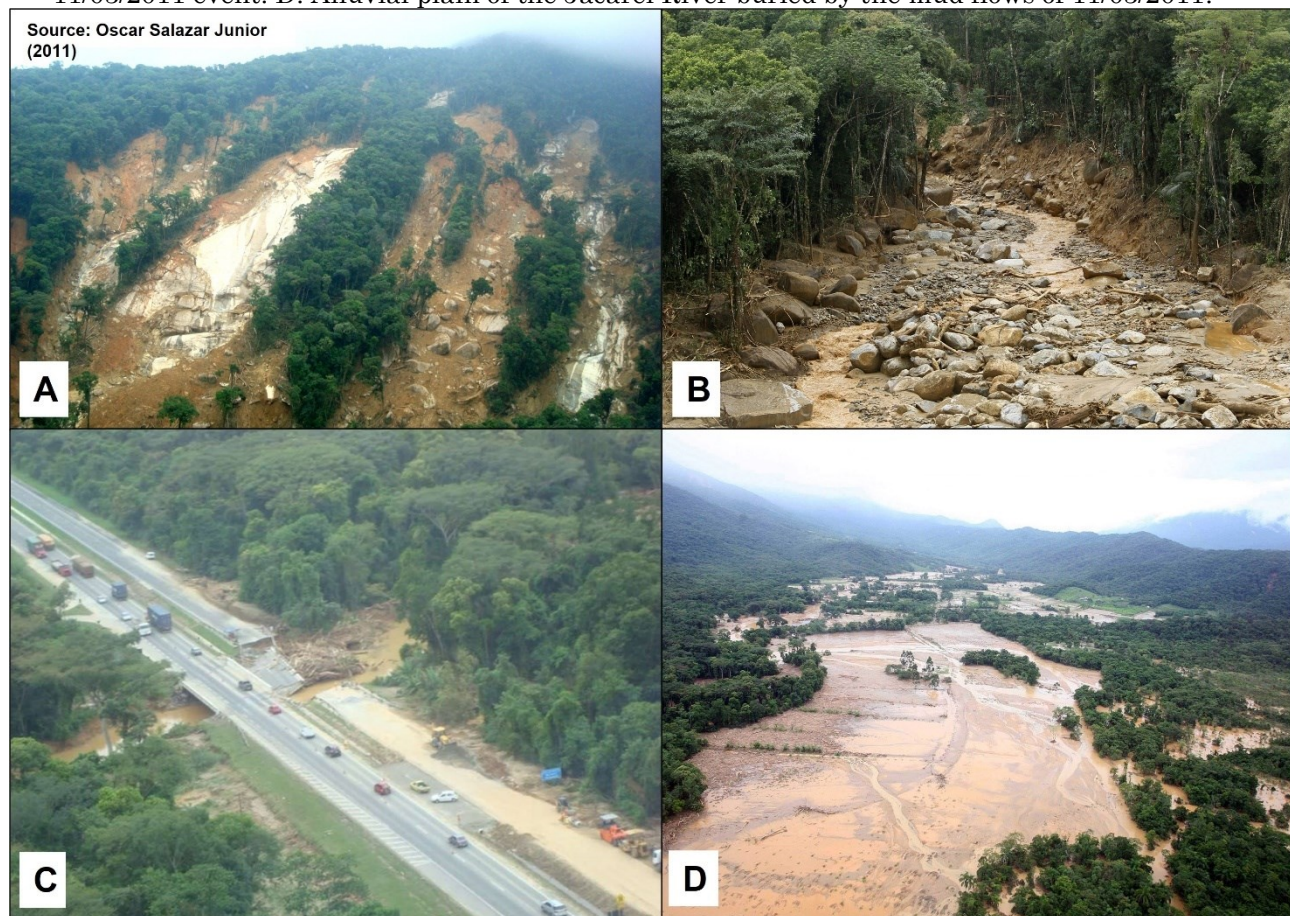
Figure 3 – A: Landslides in the upper third of the slopes of the Serra da Prata. B: Intramontane channels after the passage of debris flows. C: BR 277 highway bridge over the Jacareí River after the 11/03/2011 event. D: Alluvial plain of the Jacareí River buried by the mud flows of 11/03/2011.
