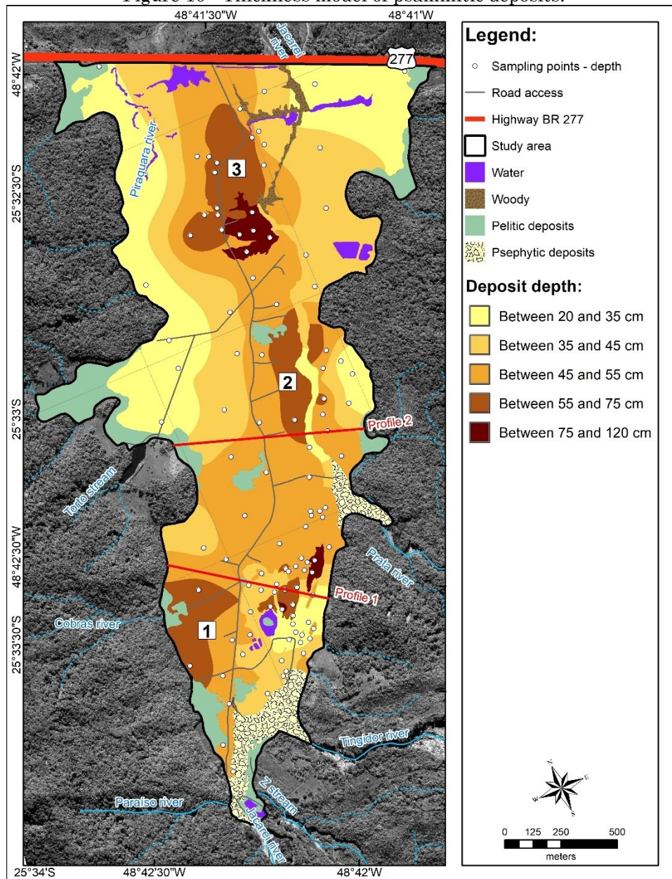
Figure 10 - Thickness model of psammitic deposits.
