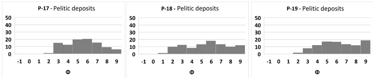
Figure 6 - Particle size frequency histogram for samples P-17 to P-19.
