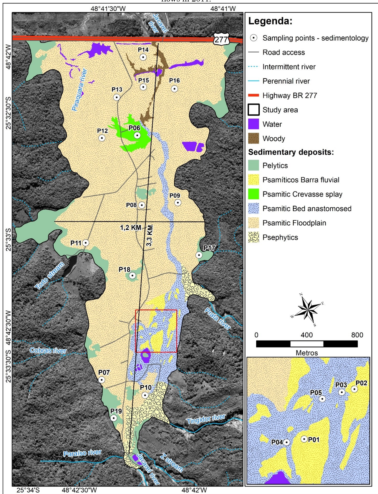
Figure 4 - Deposits in the alluvial plain of the Jacareí River in 2011. Note that the fluvial channels in the plain are not illustrated in the figure due to their filling during the burial event by the mud flows in 2011.
