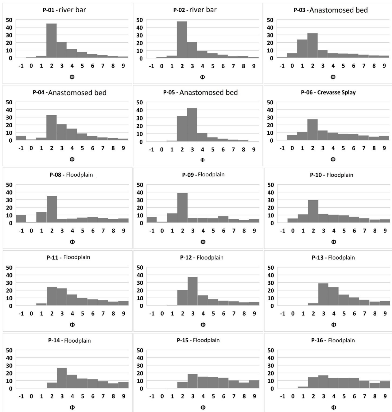
Figure 5 - Particle size frequency histogram for the samples P-01 to P-16.
