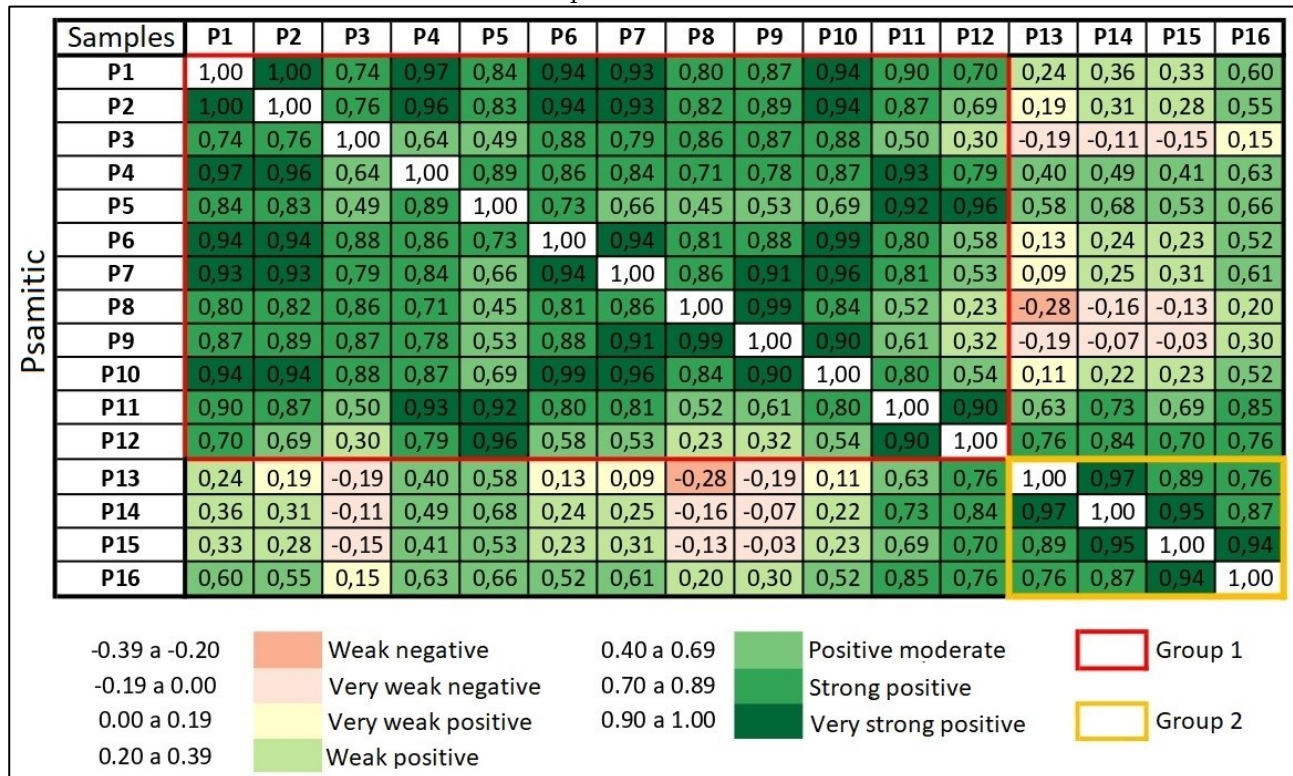
Figure 7 - Bivariate correlation matrix between the granulometric distributions of the psammitic samples collected.
