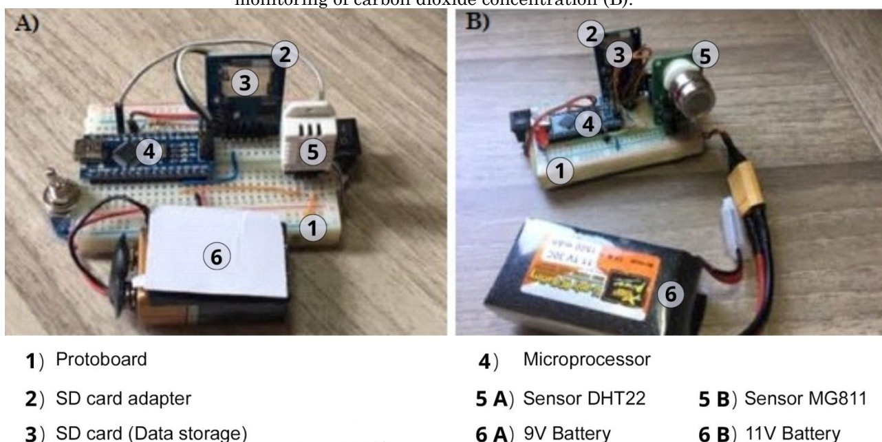
Figure 1 – Sensor nodes developed for the monitoring of the AT and the RH (A) and for the monitoring of carbon dioxide concentration (B).
