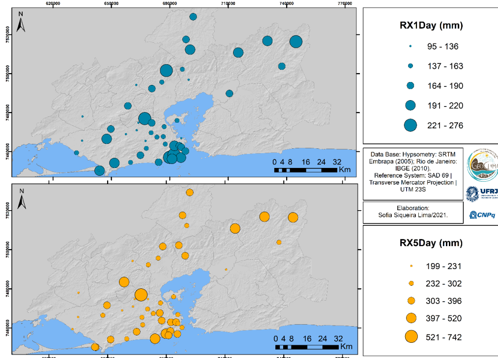
Figure 8 - Parameters RX1Day (upper) and RX5Day (lower) by rainfall station.
