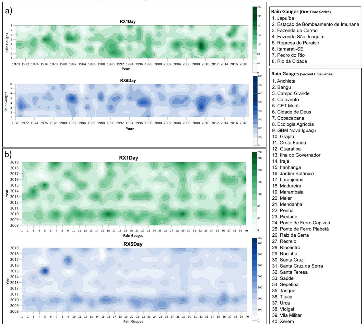
Figure 10 - Space-time panel of the annual parameters of the RClimDex: a) First historical series (1970-2019); b) Second historical series (2008-2019)
