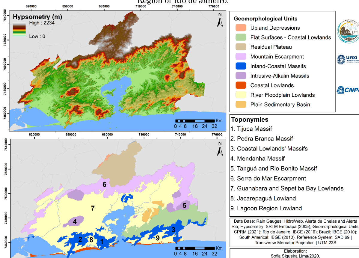
Figure 1 – Hypsometry map (upper) and geomorphological units map (lower) of the Metropolitan Region of Rio de Janeiro.
