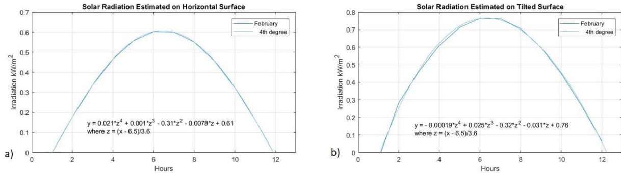
Fig. 7. Solar Radiation Estimated for Winter: a) Horizontal Surface, b) Tilted Surface.
