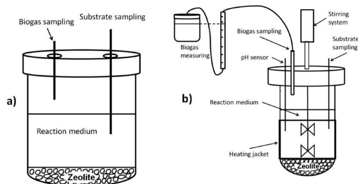
Figure 1. Schematic representation of a bioreactors: a) 120ml, b) 7 liters.
