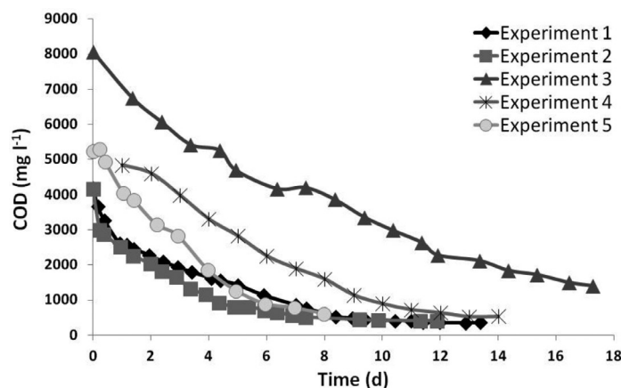
Figure 10. COD removal from batch experiments in a 7 liter reactor.
