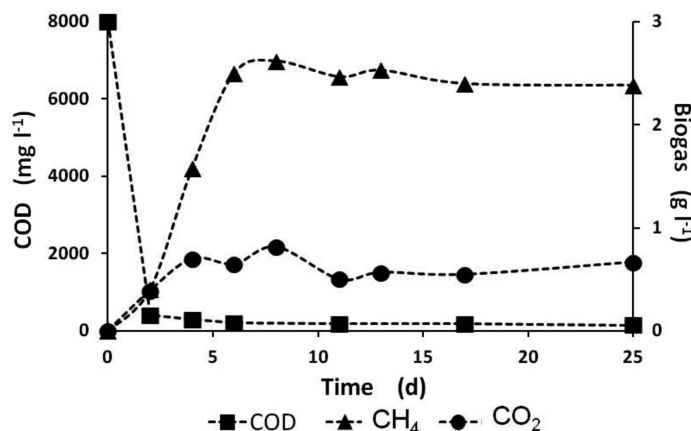
Figure 5. Process performance with biofilm: 45 days (particle size: 9-10 mesh).
