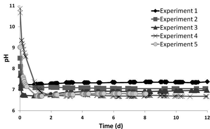
Figure 9. pH trends for batch experiments in a 7 liter reactor.
