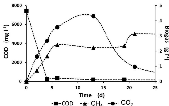
Figure 3. COD removal and methane production without biofilm (particle size: 9-10 mesh).
