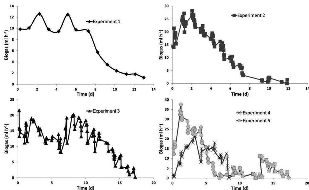
Figure 11. Biogas production from batch experiments in a 7 liter reactor.
