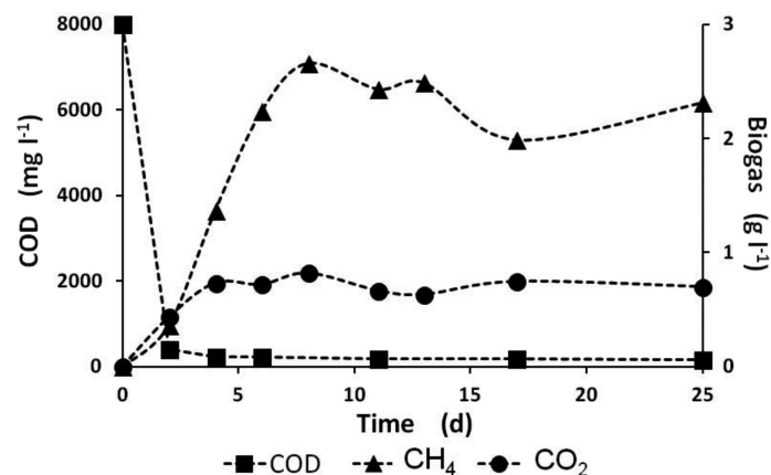
Figure 7. Process performance with biofilm: 60 days (particle size: 9-10 mesh).
