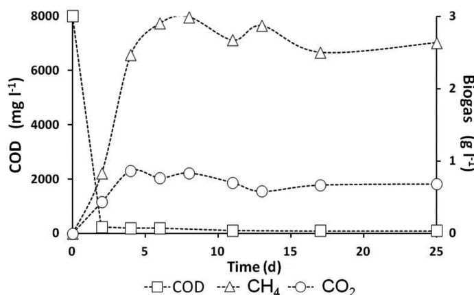
Figure 6. Process performance with biofilm: 45 days (particle size: 20-35 mesh).
