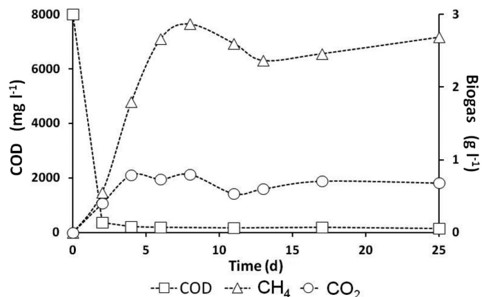
Figure 8. Process performance with biofilm: 60 days (particle size: 20-35 mesh).
