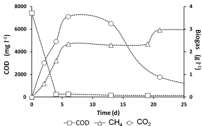
Figure 4. COD removal and \text{CH}_4 production without biofilm (particle size: 20-35 mesh).
