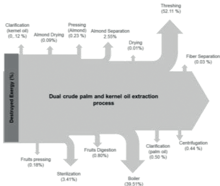
Figure 4. Sankey diagram for dual crude palm and kernel oil extraction process
