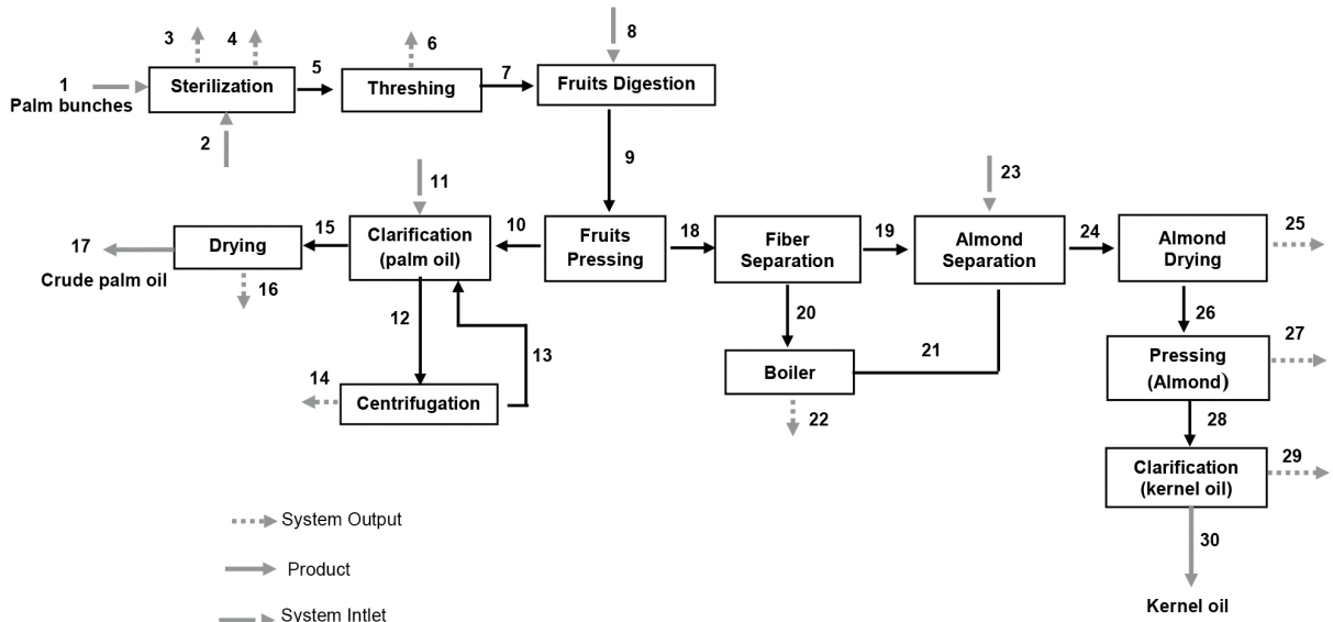
Figure 1. Block diagram of the dual crude palm and kernel oil production process.
