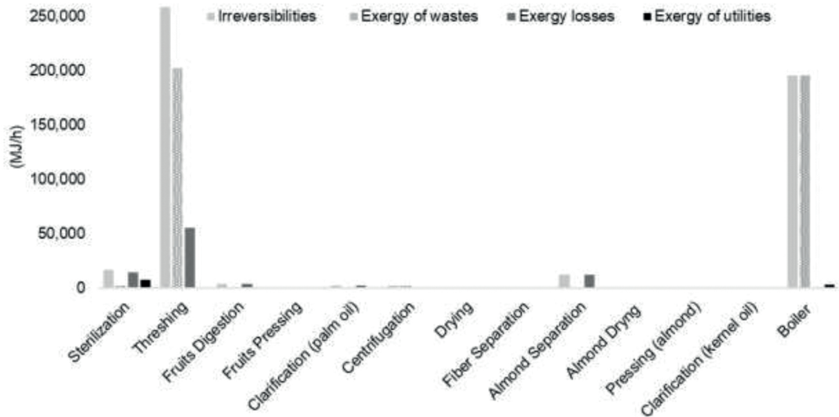
Figure 2. Exergy results for dual crude palm and kernel oil extraction process per stage.
