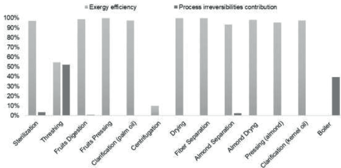
Figure 3. Exergy efficiency and contribution to exergy loss per stage
