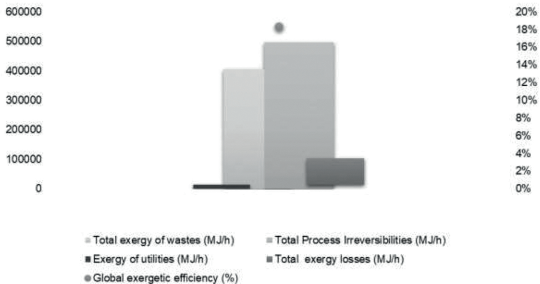
Figure 5. Global exergy results for dual crude palm and kernel oil extraction process.
