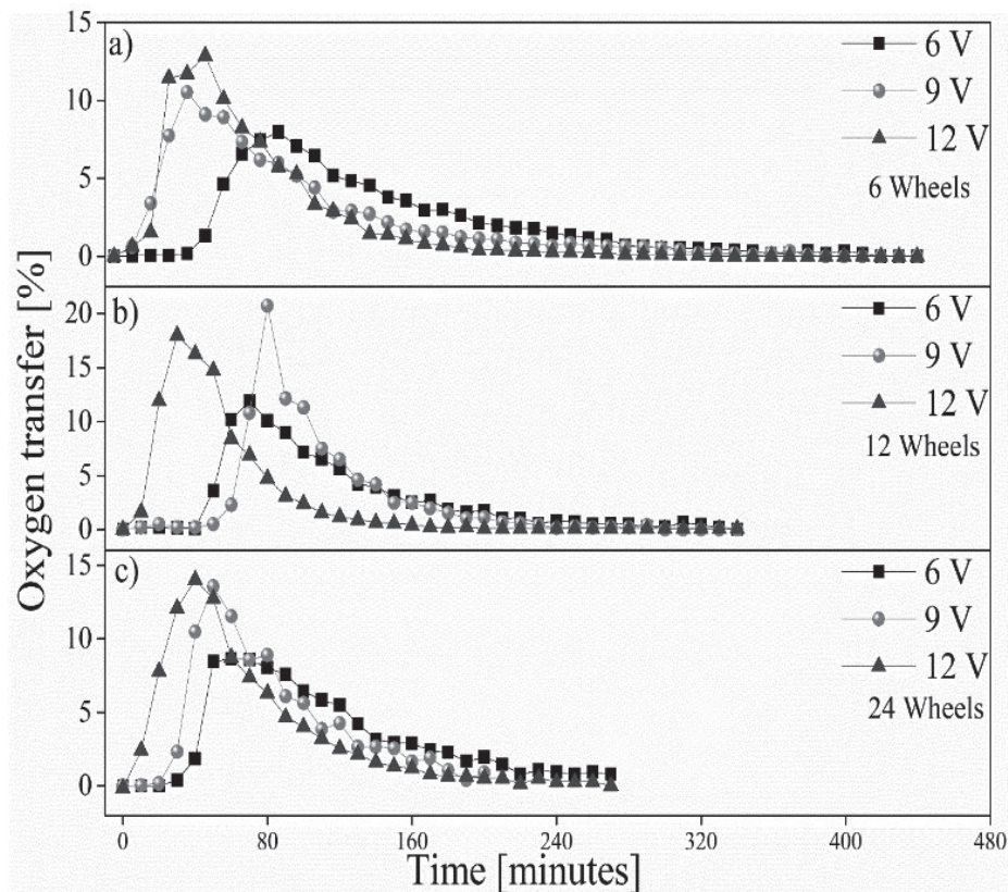
Figure 3. Percentage of oxygen transfer as a function of time for a) 6 wheels, b) 12 wheels and c) 24 wheels.
