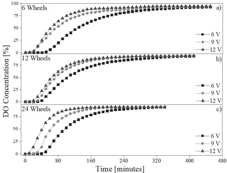
Figure 2. DO transfer percentage for aeration system of a) 6 wheels, b) 12 wheels and c) 24 wheels.
