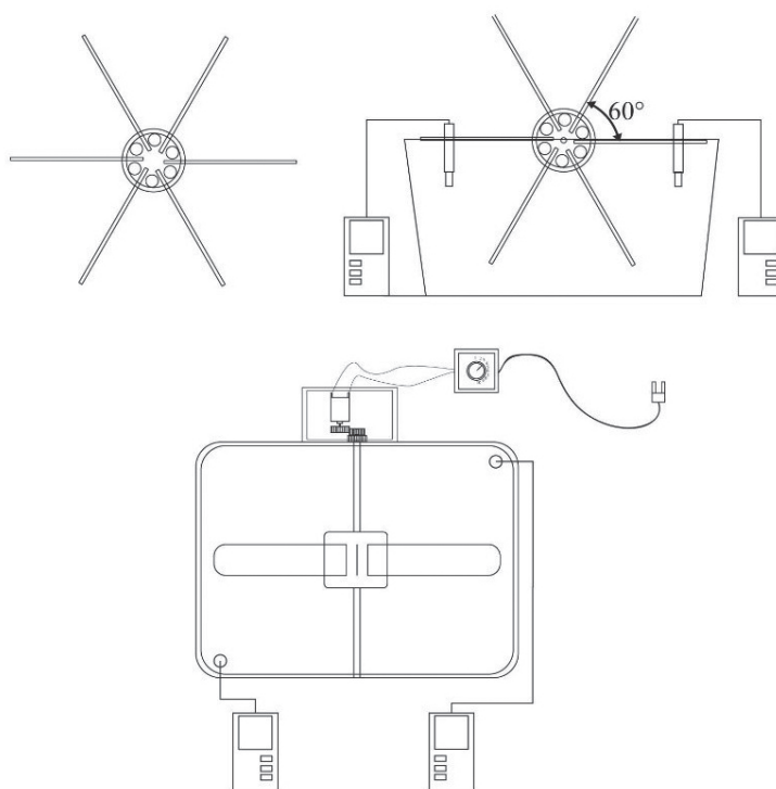
Figure 1. Experimental setup for performance evaluation of the paddle wheels system used in this study.
