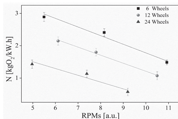
Figure 5. Energy efficiency (N) obtained in each case study.
