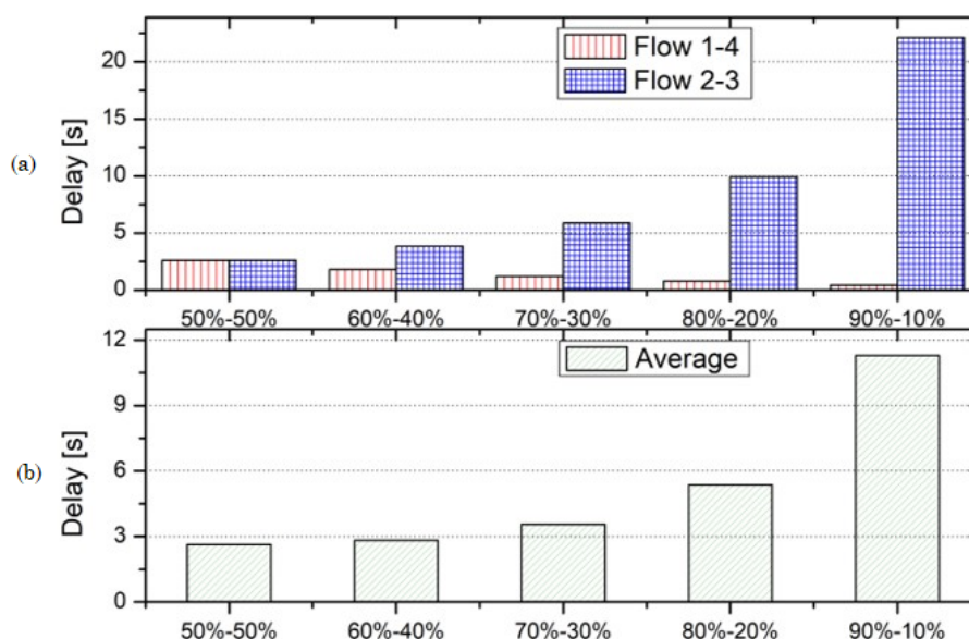
FIG. 7. Delay obtained using QoS policies. (a) Performance of individual flows. (b) Global performance. Source: Authors' own work.
