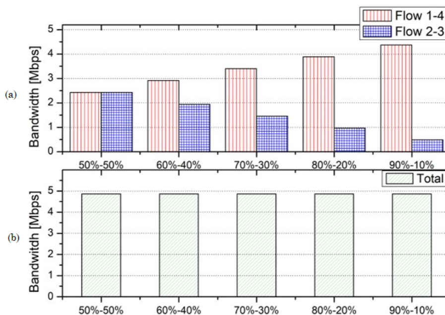
FIG. 6. Bandwidth assigned using QoS policies. (a) Performance of individual flows. (b) Global performance. Source: Authors' own work.
