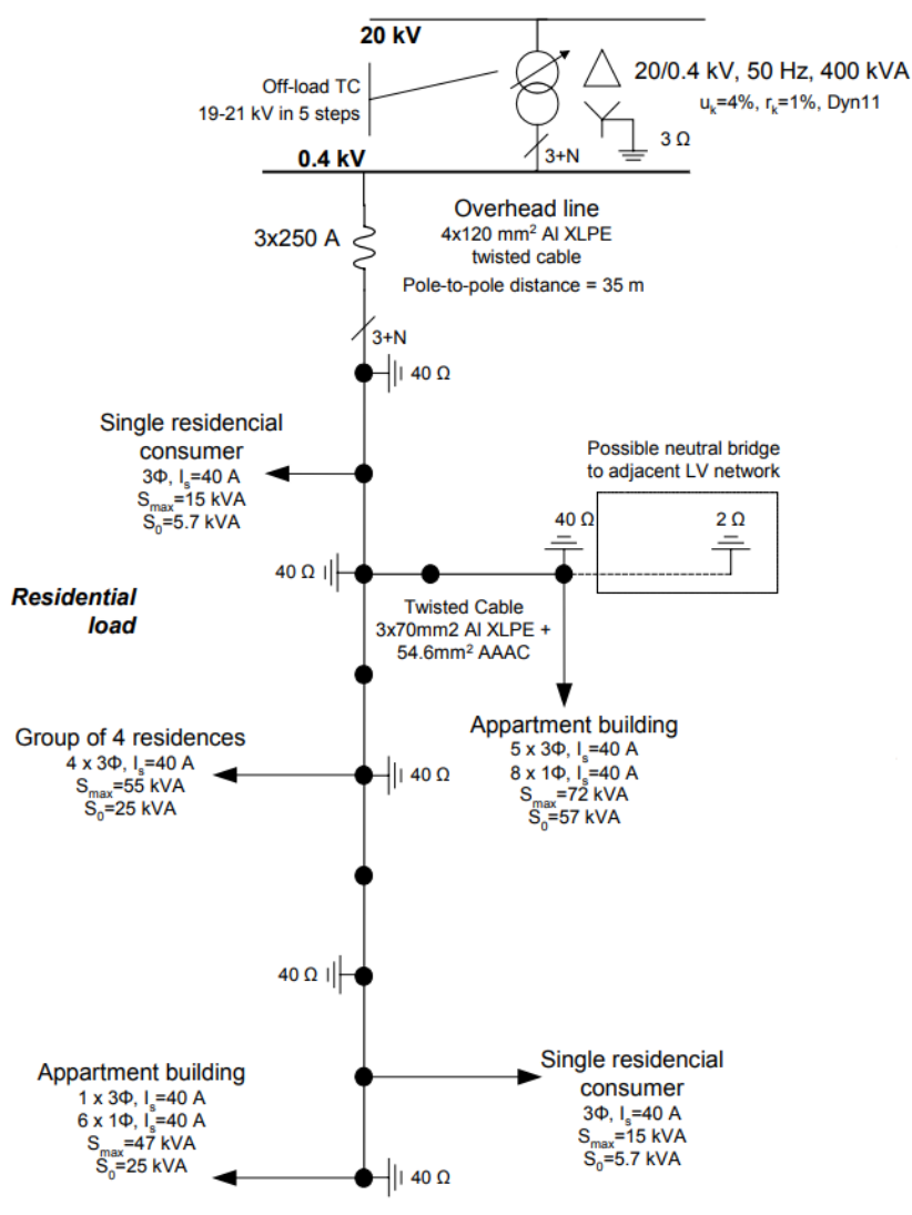
FIGURE 1. Unifilar Diagram of the CIGRE benchmark Source: Taken from [6].
