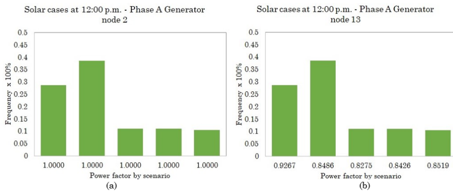
FIGURE 5. Possible power factor for phase 12 p.m.: (a) generator 1φ, node 2; (b) generator 3φ, node 13 Source: Created by authors.
