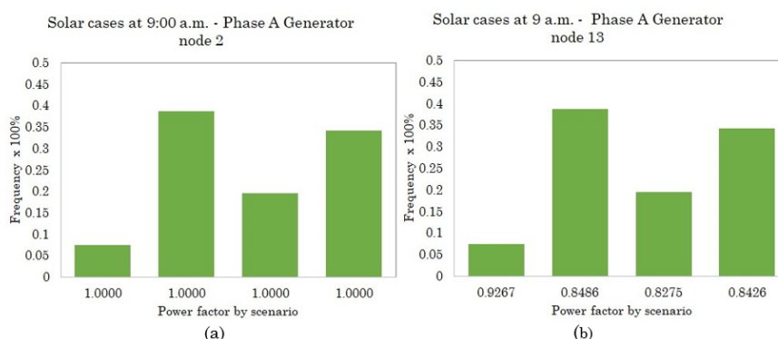
FIGURE 4. Possible power factor for phase 9 am: (a) generator , node 2; (b) generator , node 13 Source: Created by authors.
