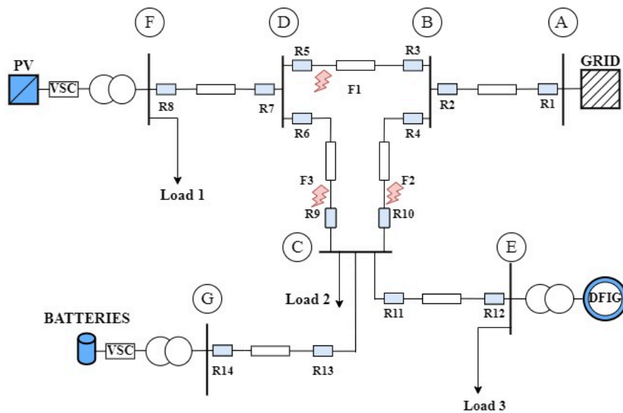
FIGURE 2. Active distributed system used as a test system Source: Created by the authors.
