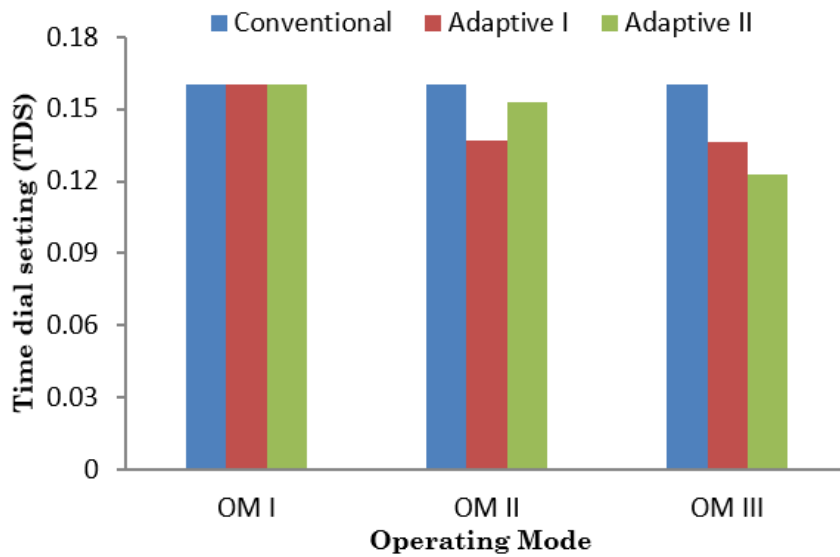
FIGURE 5. Relay R3's TDS for each operation mode
