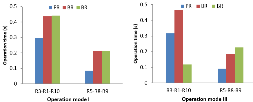
FIGURE 3. Time operation relay primary (PR) and backup (BR)
