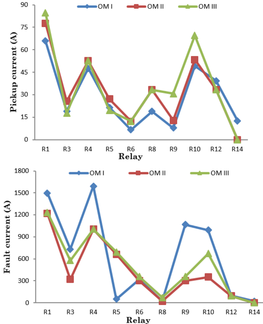
FIGURE 4. Pickup and fault current for each operation mode (OM)
