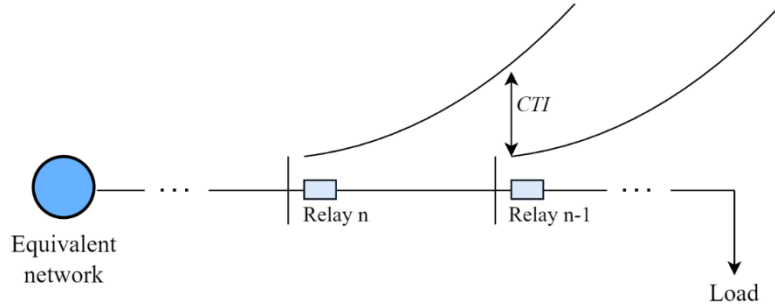
FIGURE 1. Adequately coordinated 51 relays Source: Created by the authors.
