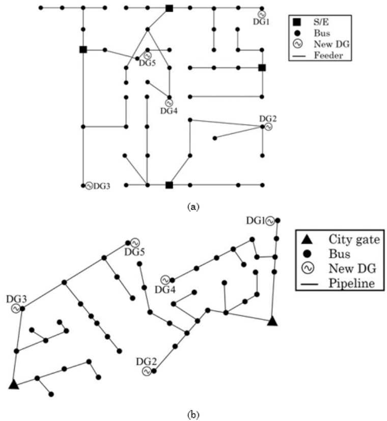
FIGURE 3. Test system: a) Electrical network b) Natural gas network
