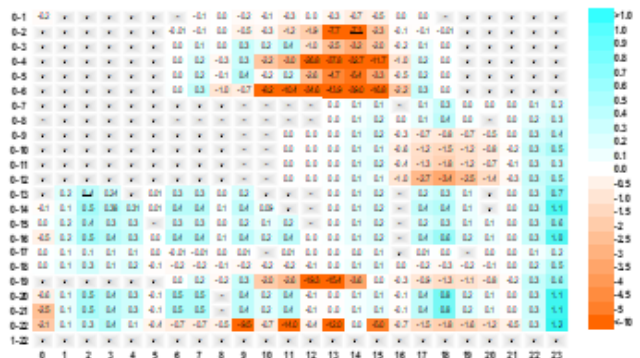
f) Power factor – Phase B
