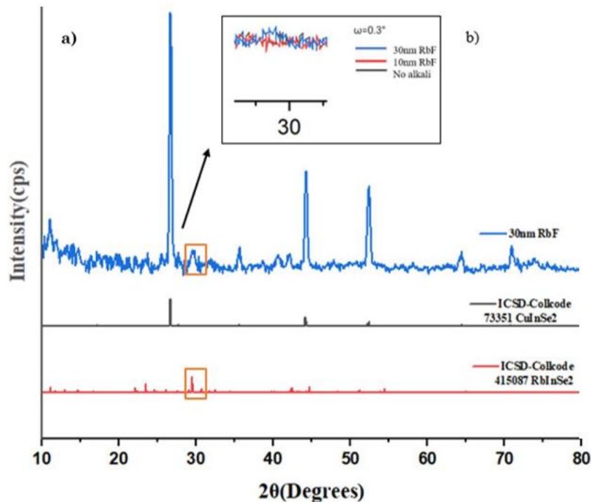
Figure 4. X-ray and b) Grazing incidence diffraction for the sample with 30nm of RbF Source: Created by the authors.
