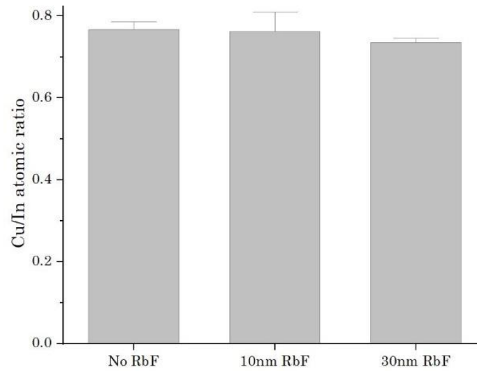
Figure 1. Elemental ratios measured using X-ray fluorescence. Source: Created by the authors.
