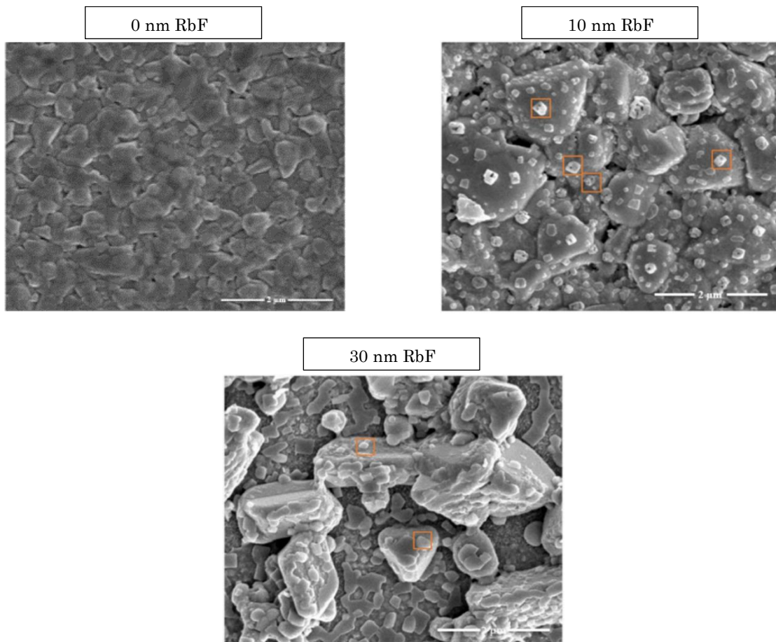
Figure 2. Top-view SEM images of CISE-based thin films with different amounts of Rubidium Fluoride addition. Source: Created by the authors.
