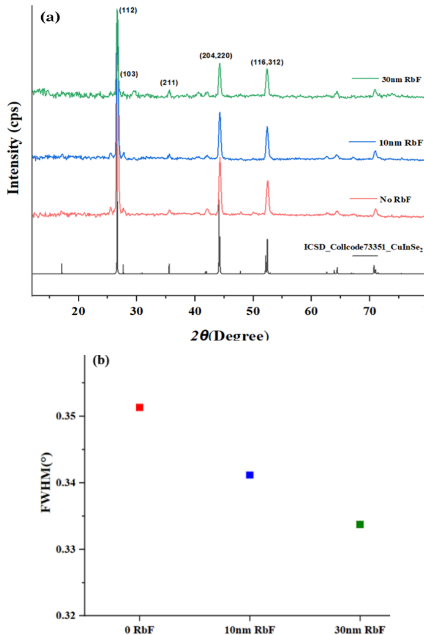
Figure 3. a) X-ray diffraction patterns of CISE samples with the addition of RbF. b) FWHM of the main diffraction plane of the CISE tetragonal structure (112). Source: Created by the authors.
