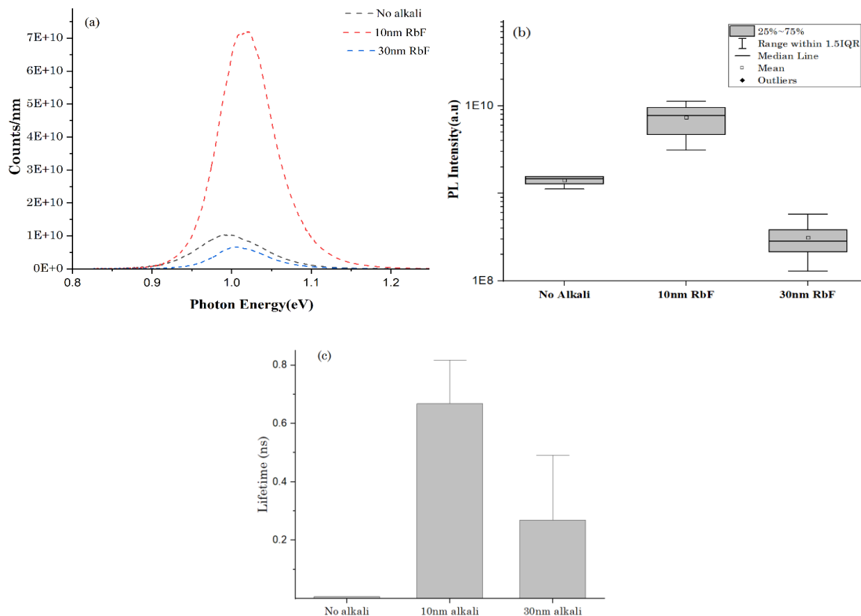
Figure 5. (a), (b) Photoluminescence signals and (c) Time-resolved photoluminescence results for CISE thin films with the addition of RbF. Source: Created by the authors.
