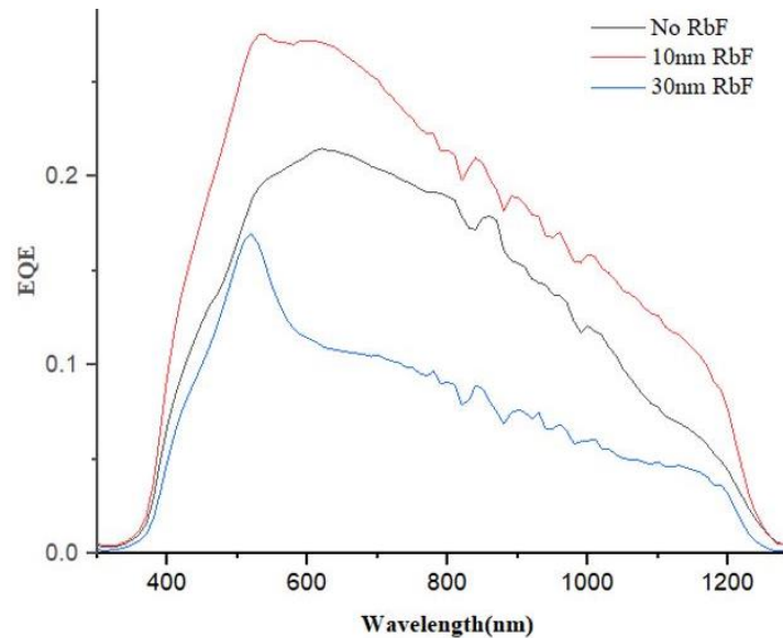
Figure 6. EQE measurements with the addition of RbF; without RbF, 10 nm RbF, and 30 nm RbF Source: created by the authors.
