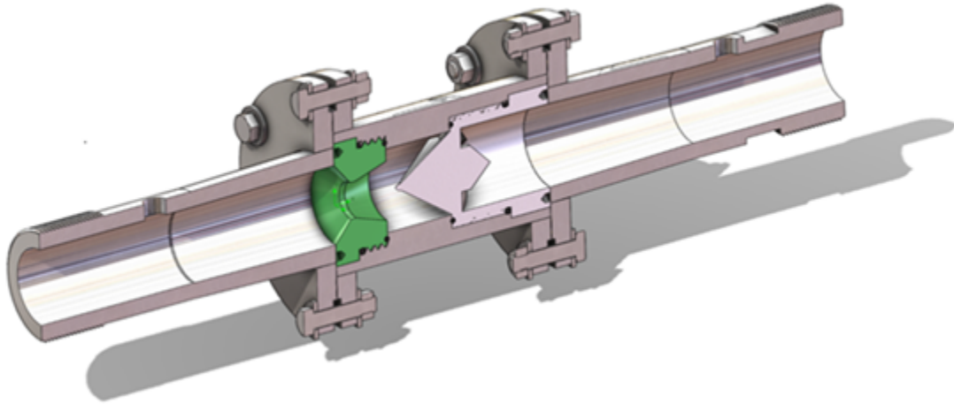
Figure 3. Geometry of a disinfection element by cavitation. Source: created by the authors.
