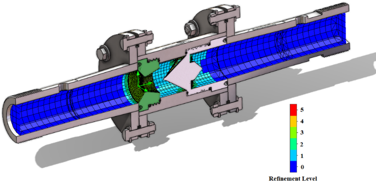
Figure 4. Discretization of the CFD model of the cavitation disinfection element. Source: created by the authors.
