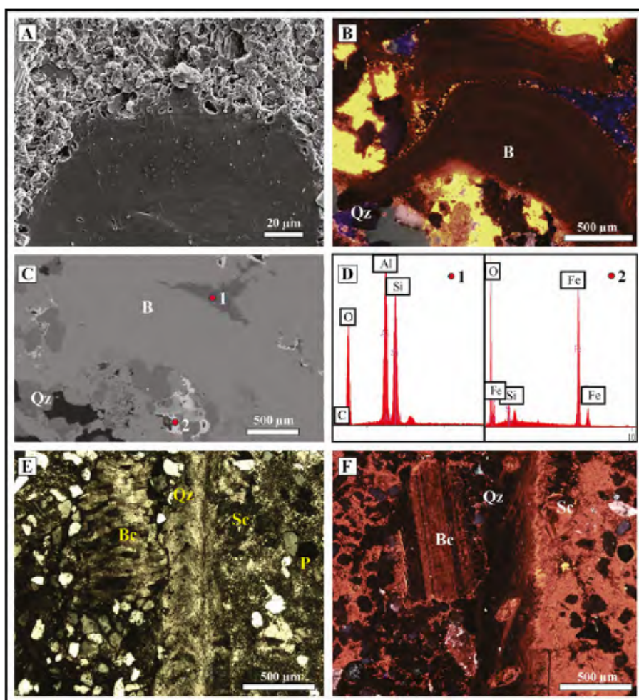
Figure 6. Cementation phases.
