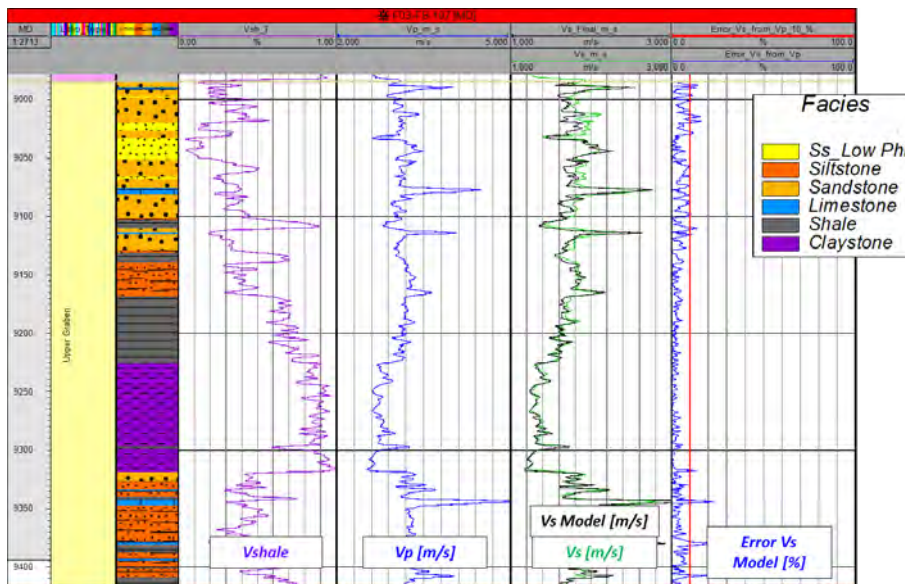
Figure 9. S-wave velocity modeled (black curve in sixth track) by using equation 1 and its corresponding error (blue curve in seventh track) compared to the original S-wave velocity log (green curve in sixth track).
