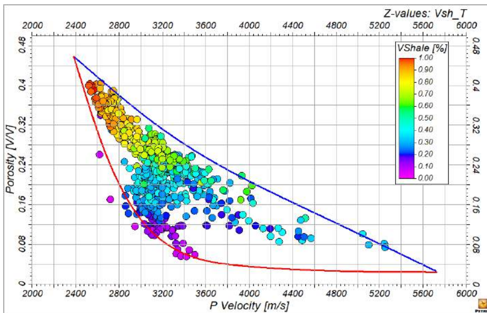
Figure 10. P-wave velocity vs total porosity crossplot along with the limits defined to use equation 2.
