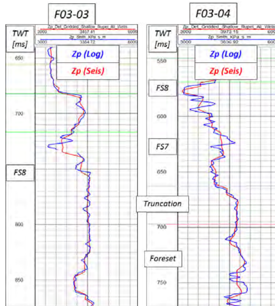
Figure 22. Comparison of the final acoustic impedance model obtained from deterministic seismic inversion (red) with the acoustic impedance model from well logs (blue) for two correlation wells.
