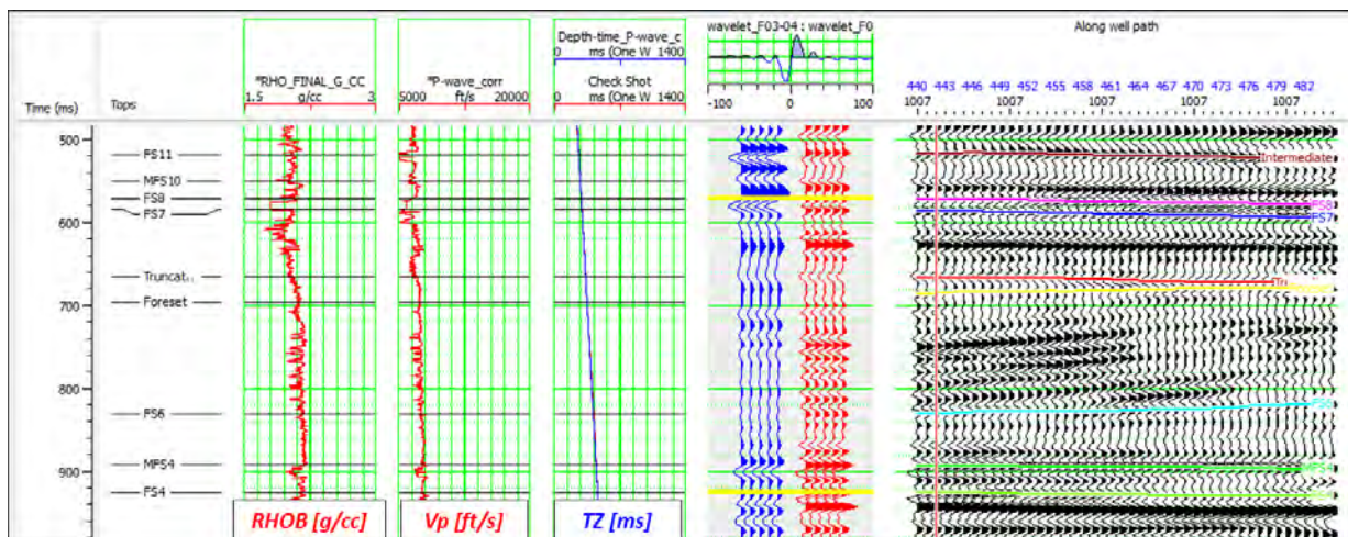
Figure 13. Resulting seismic-well tie for one of the correlation wells.
