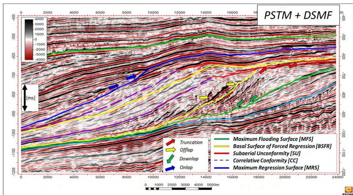
Figure 19. Seismic stratigraphic model built for the interval of interest. Taken from Illidge et al. (2016).
