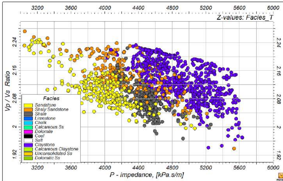
Figure 12. RPT that best contrast the sandy facies from the shaly facies for the interval of interest.
