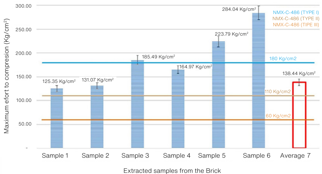
FIGURE 6. Graph of the maximum compressive strength of the samples extracted and prepared according to Mexican Standard NMX-C-038-ONNCCE-2013 (Graph: Alejandro Leal & Alberto Muciño, 2021).
