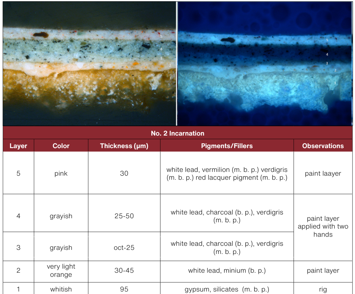
FIGURE 6. Image obtained under the optical microscope of the cross section of micro sample No. 2. Nikon Mplan 20X/0.45 objective with polarized light and UV light, as well as stratigraphic according to the chromatography of the chemical composition of each stratum (ARTE-LAB).
