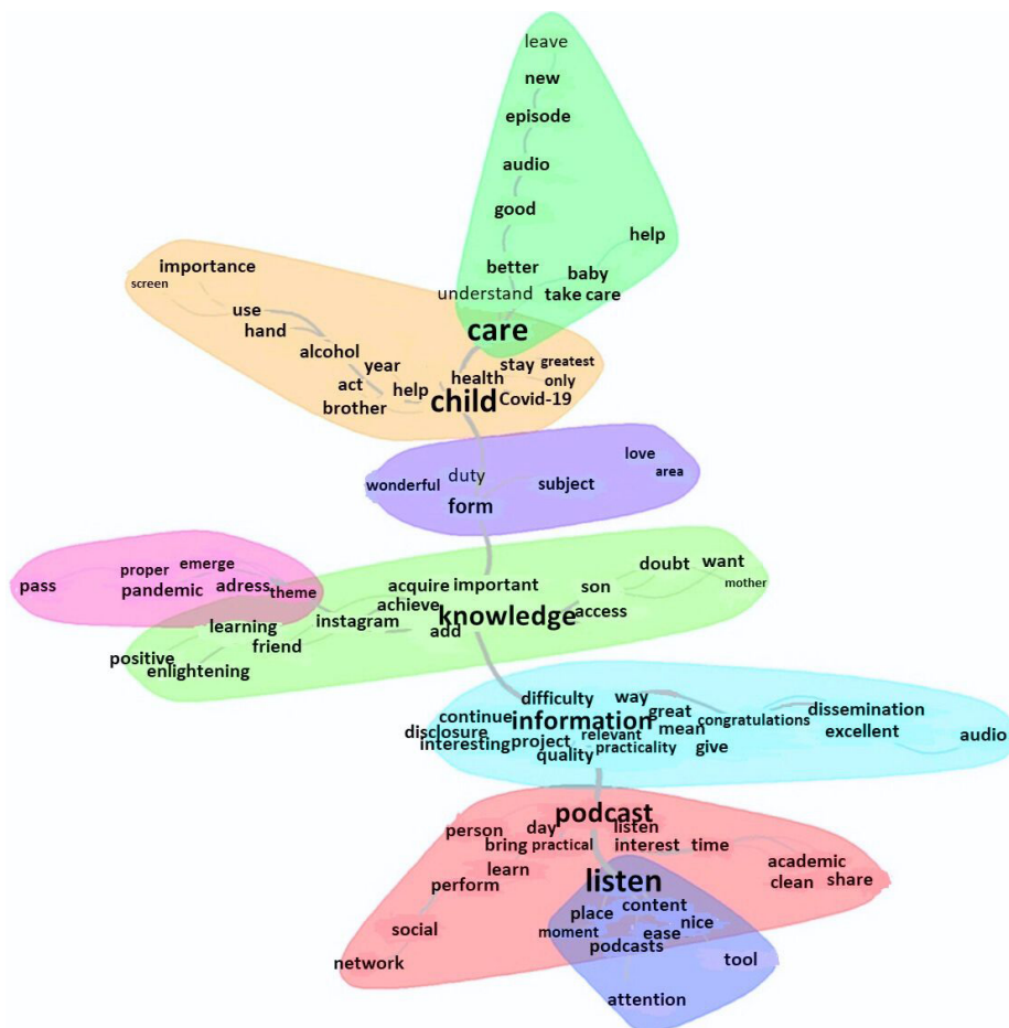
Figure 2. Similarity Analysis
