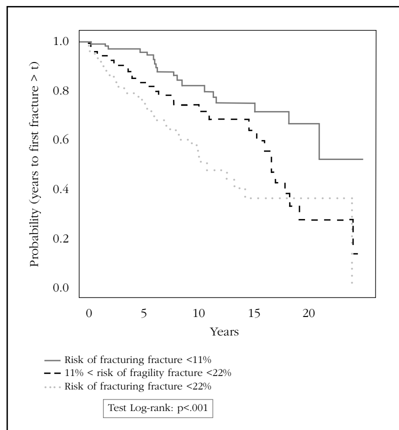
Figure 2. Survival curves up to the first fracture according to the groups defined by the tertiles of the Garvan value for risk of any fragility fracture
