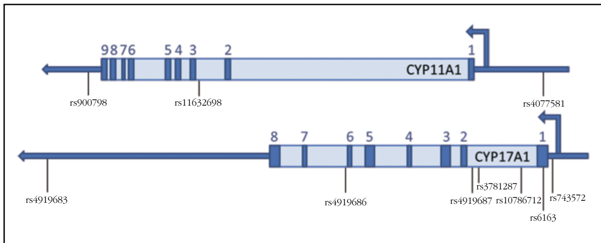
Figure 1. SNPs selected for the construction of haplotypes
