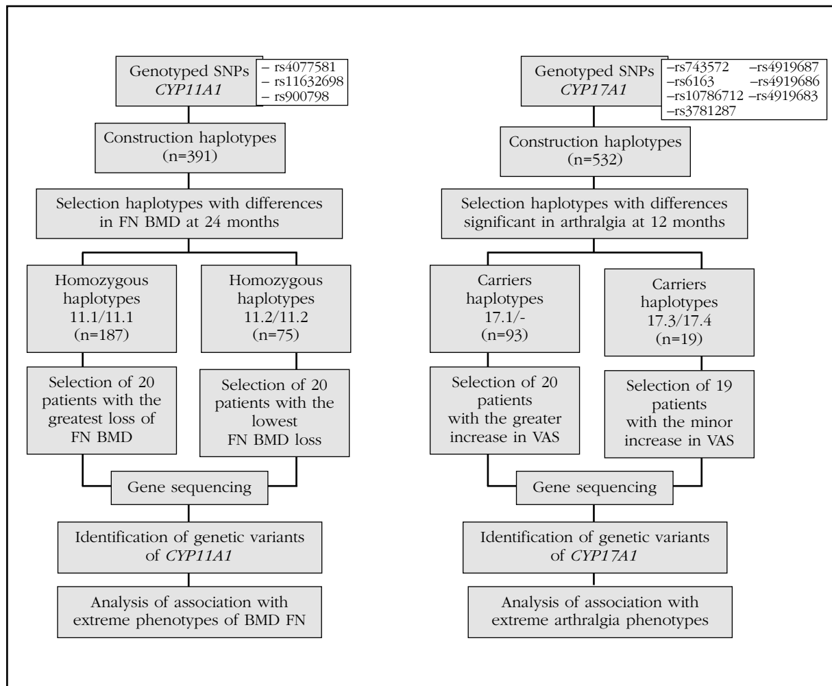
Figure 2. General outline of the association analysis process performed in the study
