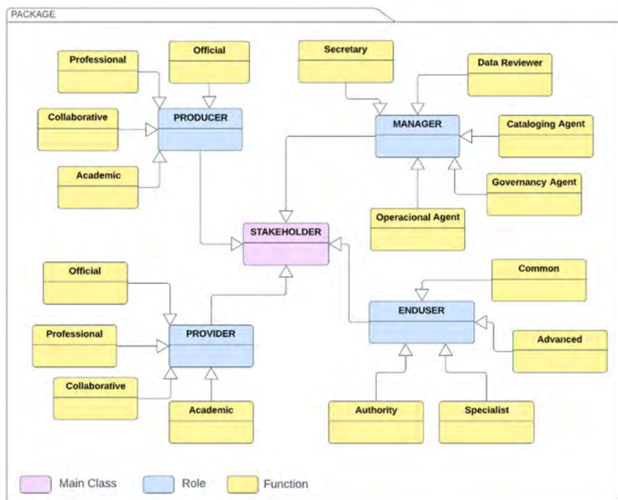
Figure 4: UML Class Diagram in the formal model, adapted from Coetzee et al. (2017) and extended for the IDE-AMB
