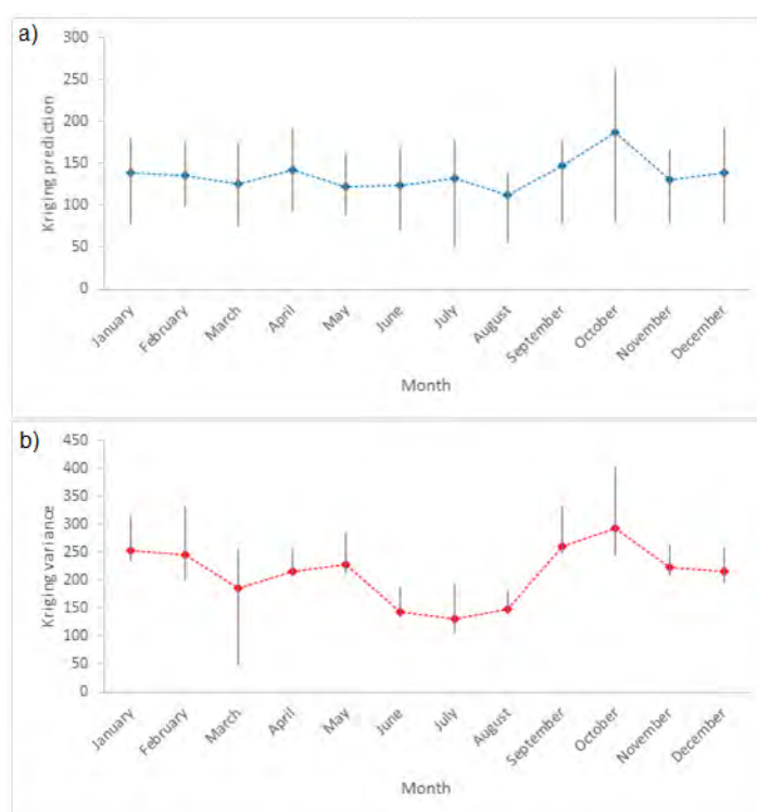
Figure 4: Behavior of kriging prediction (mean and amplitude) (mm) (a) and kriging variance (mean and amplitude) (mm 2 ) (b), in each month of the year, in the state of Rio Grande do Sul.
