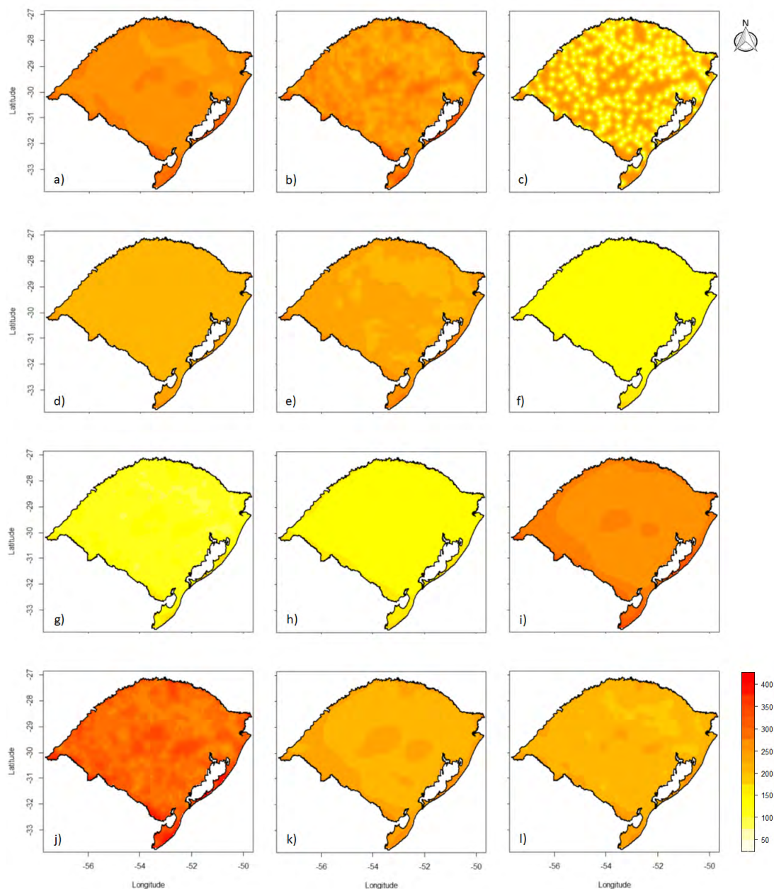
Figure 3: Kriging variance maps of the rainfall ( \text{mm}^2 ) for the months of January (a), February (b), March (c), April (d), May (e), June (f), July (g), August (h), September (i), October (j), November (k) and December (l).
