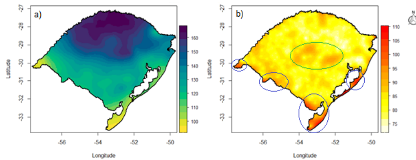
Figure 5: Average map of the kriging prediction (mm) (a), average map of the kriging variance (mm 2 ) and location of candidate sites to receive pluviometric stations (b).
