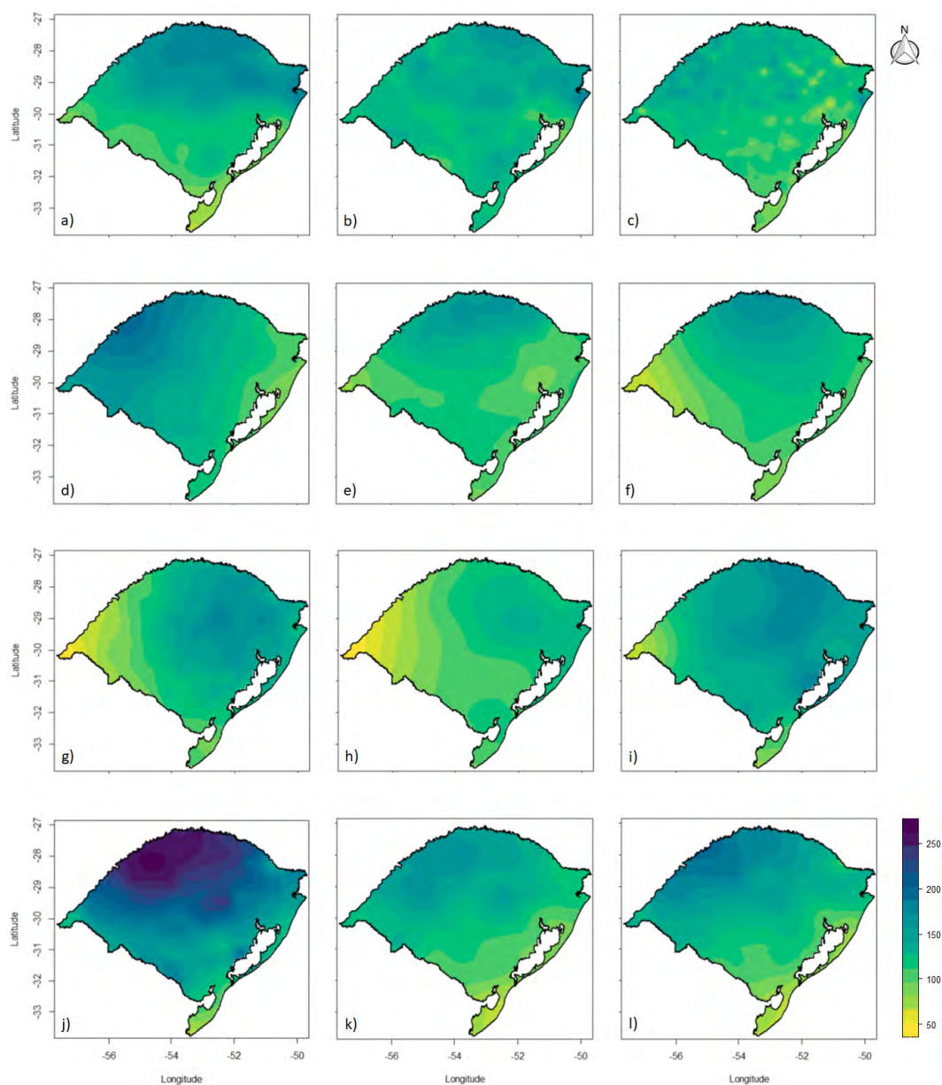
Figure 2: Kriging maps of the rainfall (mm) for the months of January (a), February (b), March (c), April (d), May (e), June (f), July (g), August (h), September (i), October (j), November (k) and December (l).
