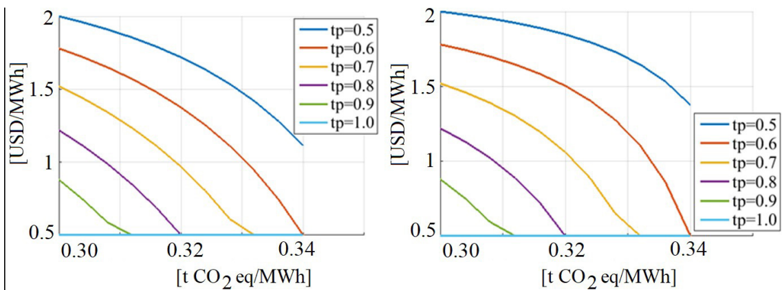
Figure 5. Investment Cost vs. Emissions for the Particular Hamacher's Product (PHP). Source: The author.
