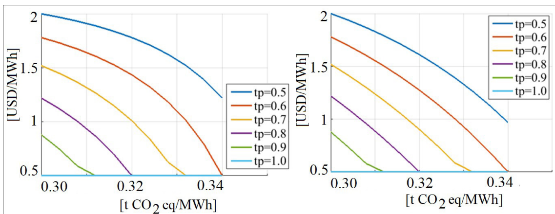
Figure 6. Investment Cost vs. Emissions for the Einstein's Product. Source: The author.
