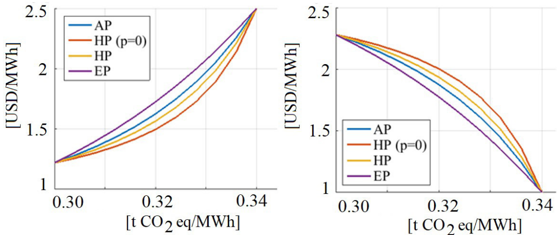
Figure 9. Left graph: Investment Cost (increase) vs. CO_2 (decrease). Right graph: Investment Cost (decrease) vs. CO_2 (decrease). Source: The author.
