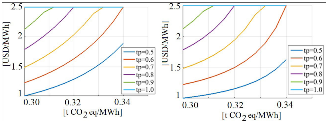
Figure 3. Investment Cost vs. Emissions for the Algebraic Product and Particular Hamacher Product. Source: The author.
