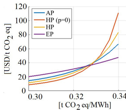
Figure 10. Intrinsic Cost vs. CO_2 Emissions (both cases: Figure 9). Source: The author.
