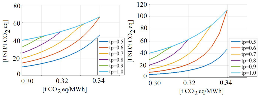
Figure 7. Investment Cost vs. Emissions for the Algebraic Product and Particular Hamacher's Product. Source: The author.
