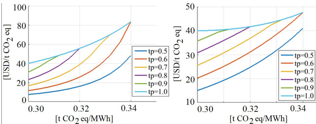
Figure 8. Investment Cost vs. Emissions for the General Hamacher's Product and Einstein's Product. Source: The author.
