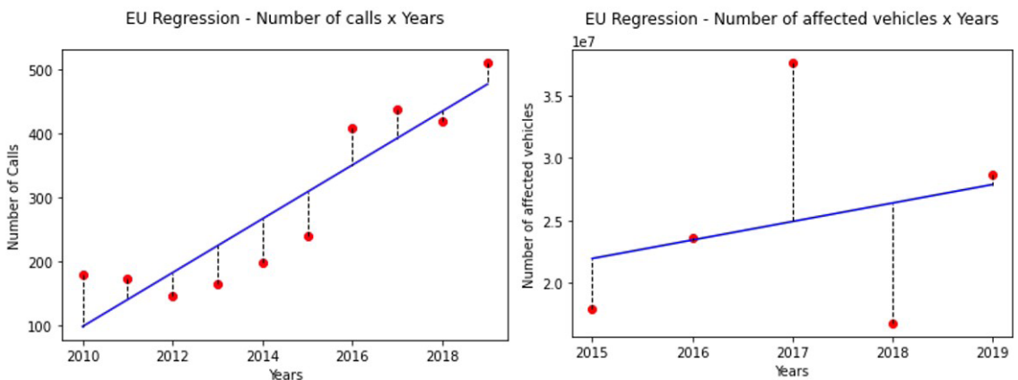
Figure 8. Regression result for the first analysis with European Union data.
