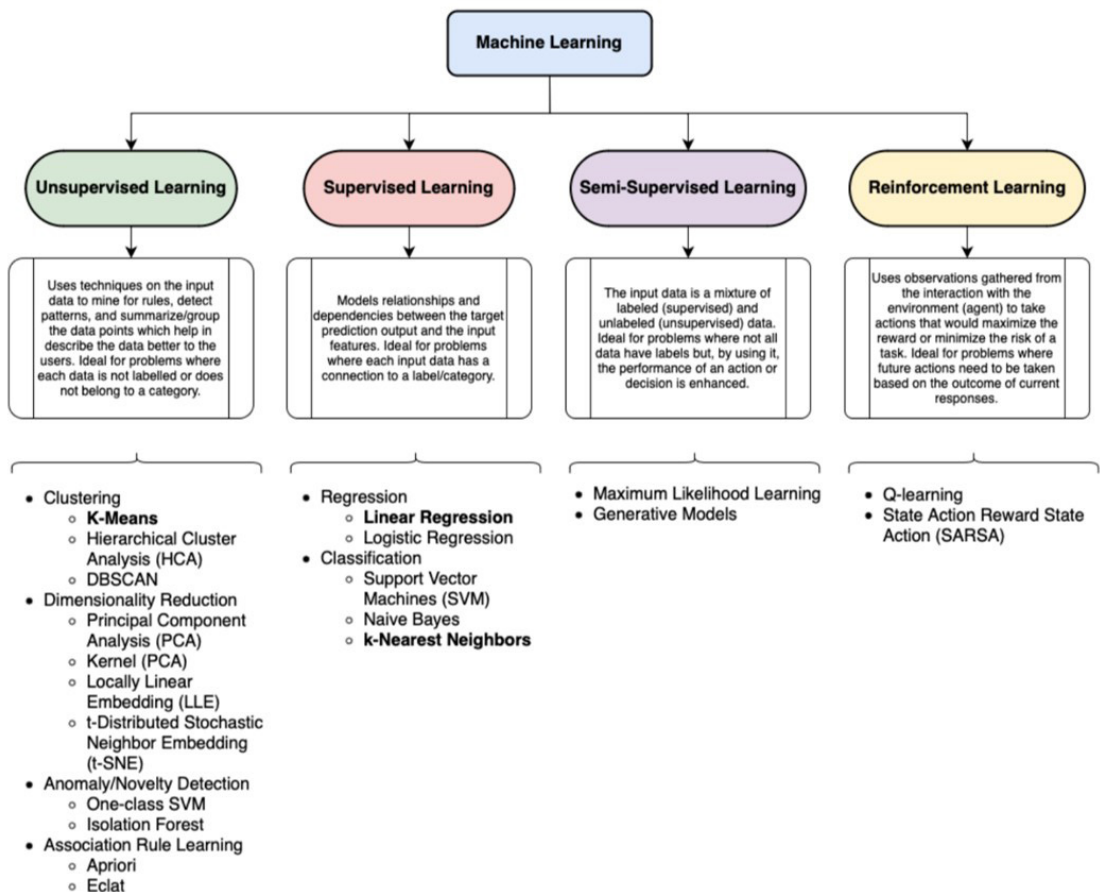
Figure 2. Flowchart of machine learning techniques. Source: Adapted from Rafique & Velasco (2018) and Géron (2019).
